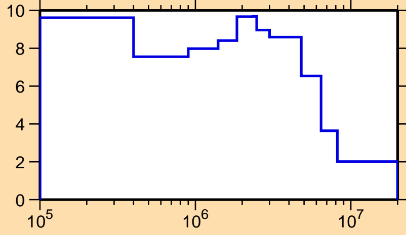
\Delta\sigma/\sigma vs. E for ^{242}\text{Am}(n,n\text{onel.})
