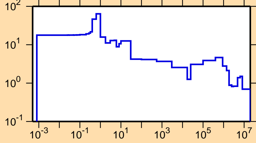
\Delta\sigma/\sigma vs. E for ^{242}\text{Am}(n,\text{tot.})
