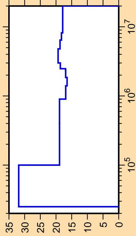
\Delta\sigma/\sigma vs. E for ^{242}\text{Am}(n,n_3)
