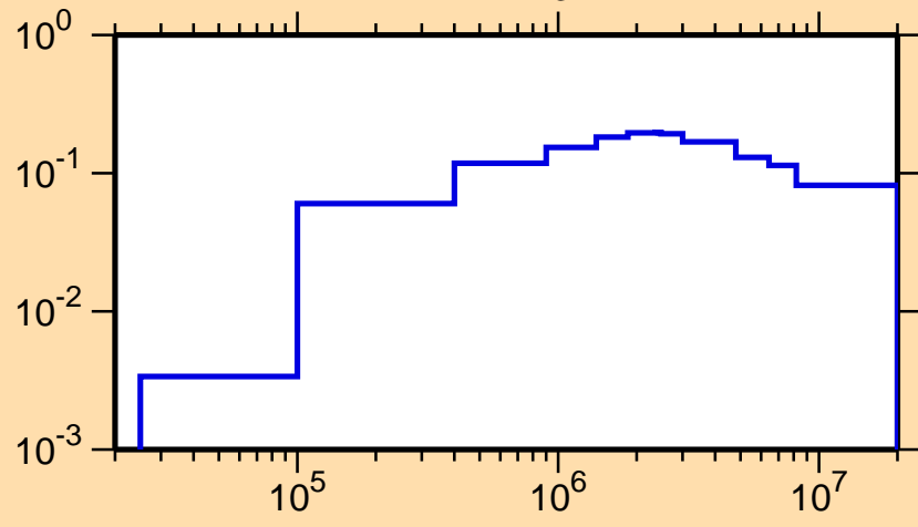
\sigma vs. E for ^{242}\text{Am}(n,n_3)
