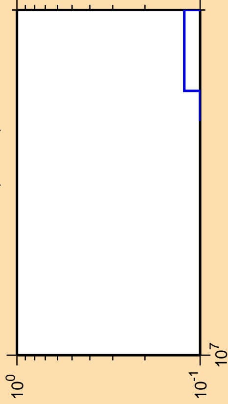
\Delta\sigma/\sigma vs. E for ^{242}\text{Am} (mt 42)
