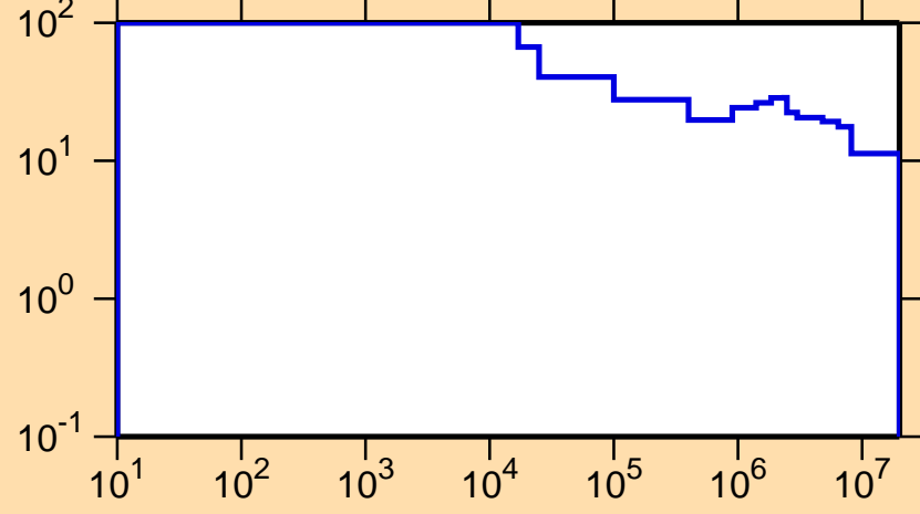
\Delta\sigma/\sigma vs. E for ^{242}\text{Am}(n,\text{nonel.})
