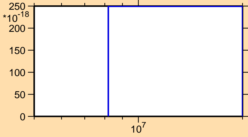
\sigma vs. E for ^{242}\text{Am} (mt 42)
