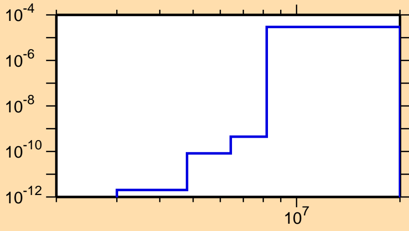
\sigma vs. E for ^{242}\text{Am}(n,\alpha)
