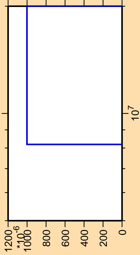
\Delta\sigma/\sigma vs. E for ^{242}\text{Am} (mt 42)
