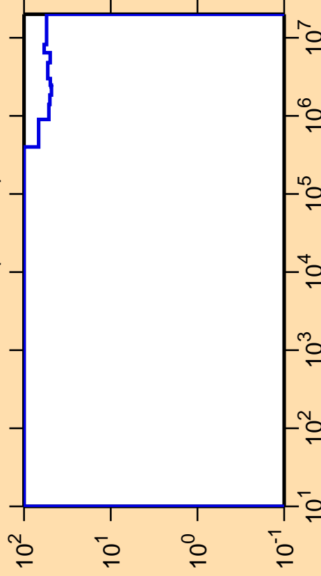
\Delta\sigma/\sigma vs. E for ^{242}\text{Am}(n,\text{inel.})
