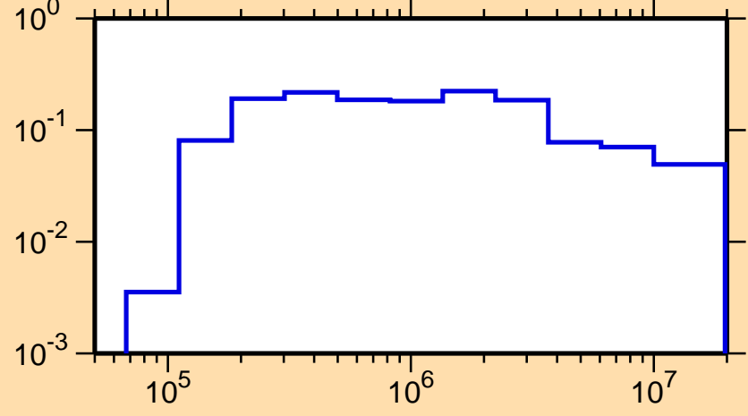
\sigma vs. E for ^{243}\text{Am}(n,n_3)
