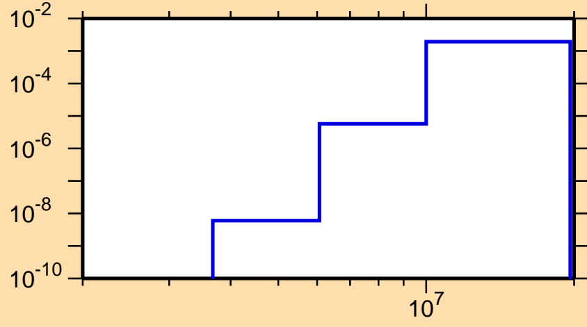
\sigma vs. E for ^{243}\text{Am}(n,p)
