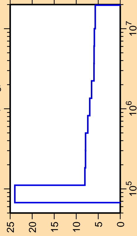
\Delta\sigma/\sigma vs. E for ^{243}\text{Am}(n,n_3)
