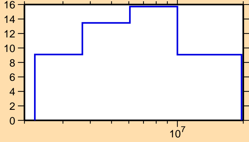
\Delta\sigma/\sigma vs. E for ^{243}\text{Am}(n,ncont.)
