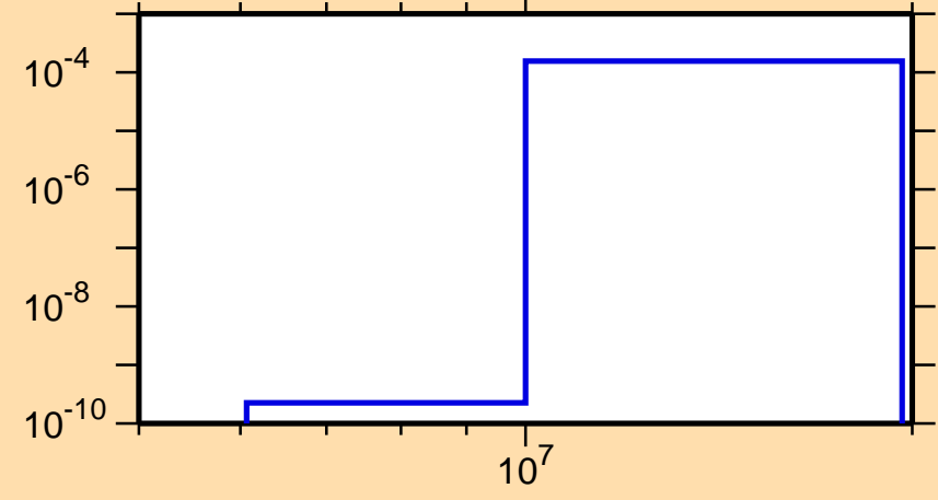
\sigma vs. E for ^{243}\text{Am}(n,np)
