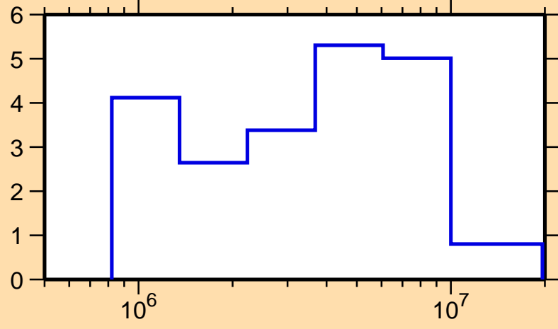
\Delta\sigma/\sigma vs. E for ^{243}\text{Am}(n,f)
