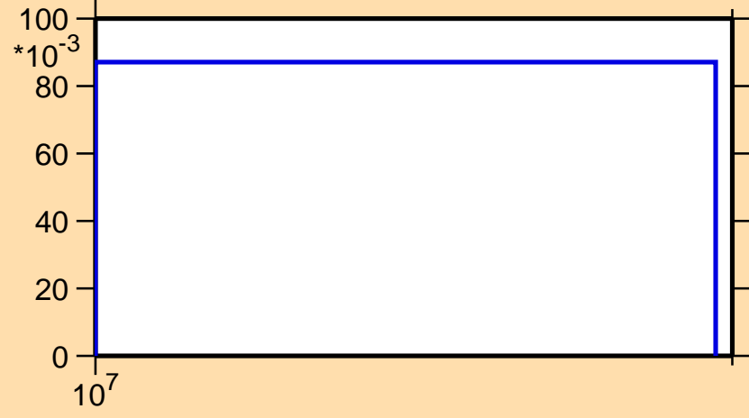
\sigma vs. E for ^{243}\text{Am}(n,3n)
