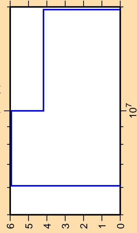
\Delta\sigma/\sigma vs. E for ^{243}\text{Am}(n,np)
