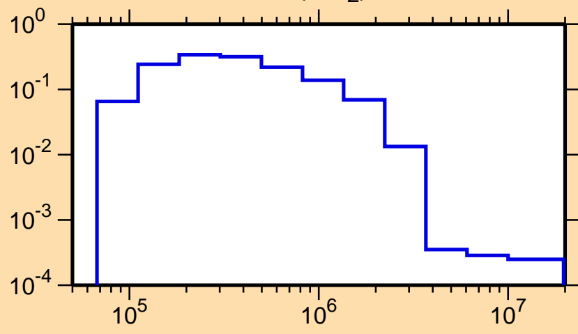
\sigma vs. E for ^{243}\text{Am}(n,n_2)
