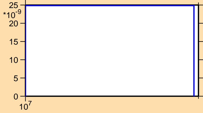
\sigma vs. E for ^{243}\text{Am}(n,\text{nd})
