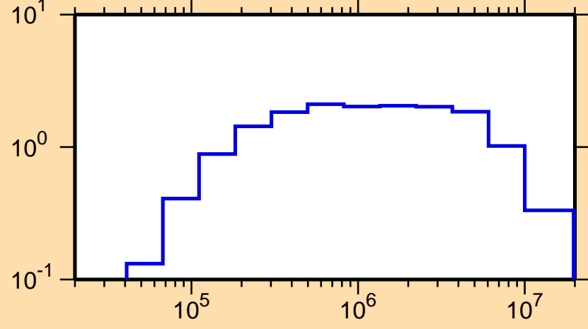
\sigma vs. E for ^{243}\text{Am}(n,\text{inel.})
