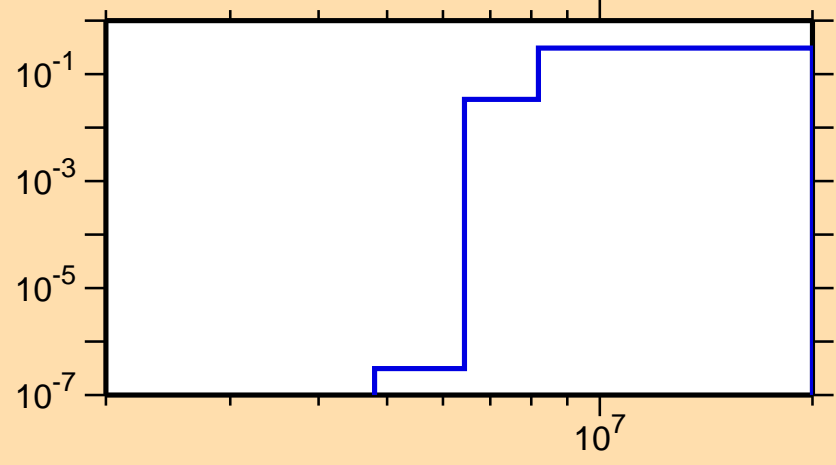
\sigma vs. E for ^{243}\text{Am}(n,2n)
