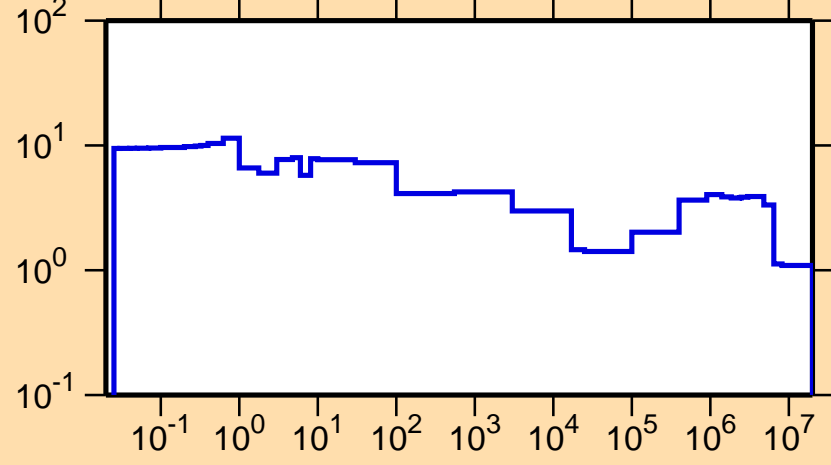
\Delta\sigma/\sigma vs. E for ^{243}\text{Am}(n,\text{el.})
