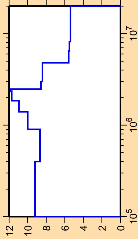
\Delta\sigma/\sigma vs. E for ^{243}\text{Am}(n,n_4)
