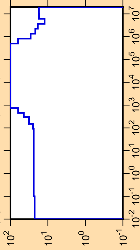
\Delta\mu/\mu vs. E for ^{244}\text{Am}(\text{mt251})
