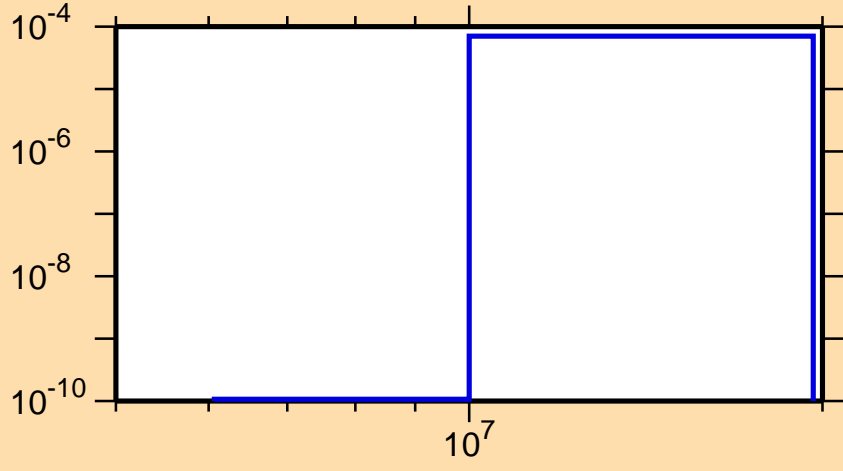
\sigma vs. E for ^{244}\text{Am}(n,t)
