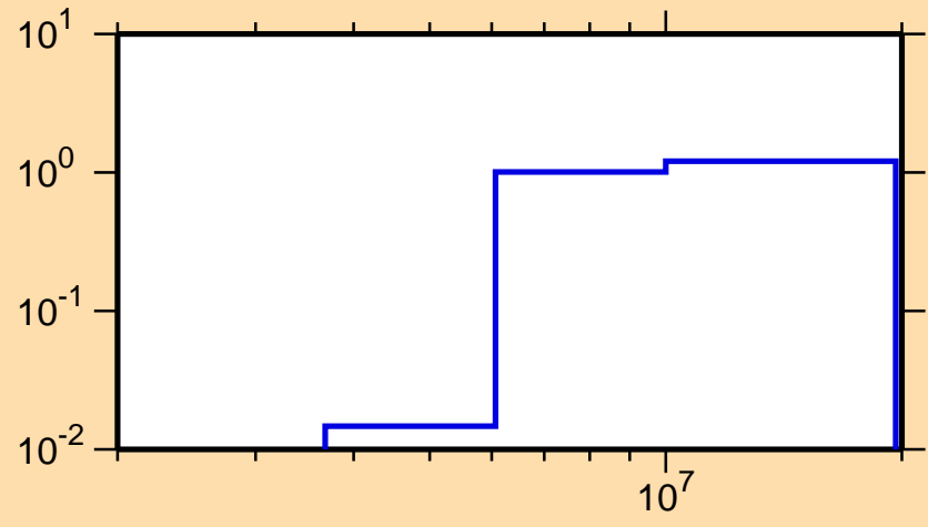
\sigma vs. E for ^{244}\text{Am}(n,2n)
