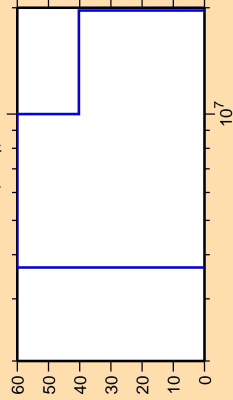
\Delta\sigma/\sigma vs. E for ^{244}\text{Am}(n,n_1)
