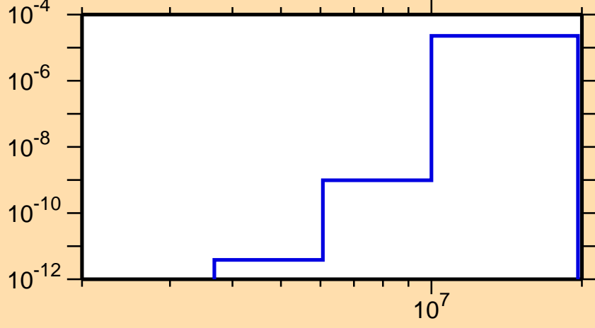
\sigma vs. E for ^{244}\text{Am}(n,n\alpha)
