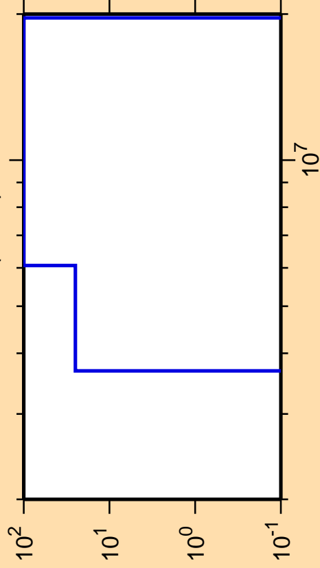
\Delta\sigma/\sigma vs. E for ^{244}\text{Am}(n,n\alpha)
