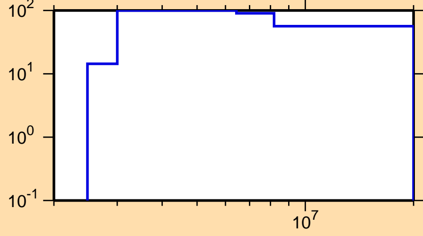
\Delta\sigma/\sigma vs. E for ^{244}\text{Am}(n,p)
