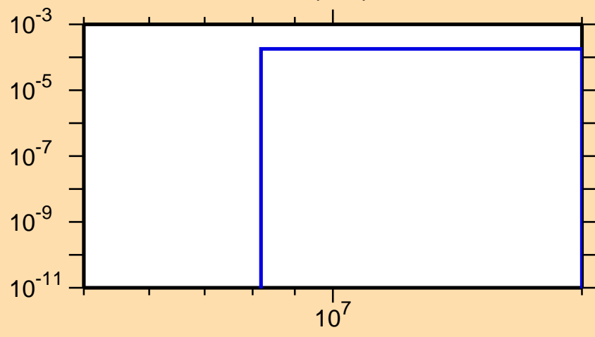
\sigma vs. E for ^{244}\text{Am}(n,d)
