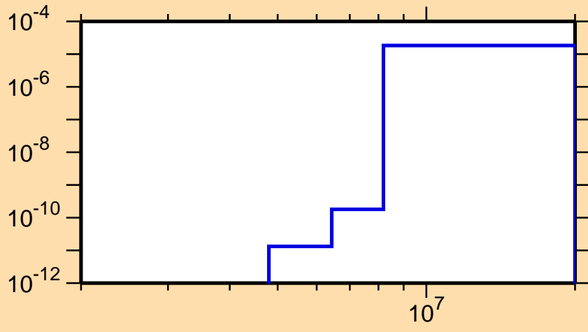
\sigma vs. E for ^{244}\text{Am}(n,n\alpha)
