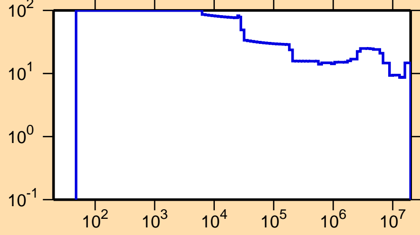
\Delta\sigma/\sigma vs. E for ^{244}\text{Am}(n,\text{tot.})
