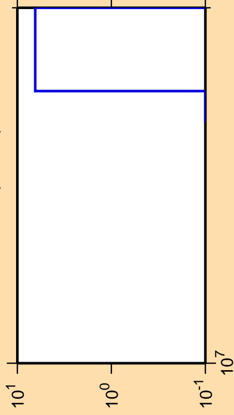
\Delta\sigma/\sigma vs. E for ^{244}\text{Am} (mt 11)
