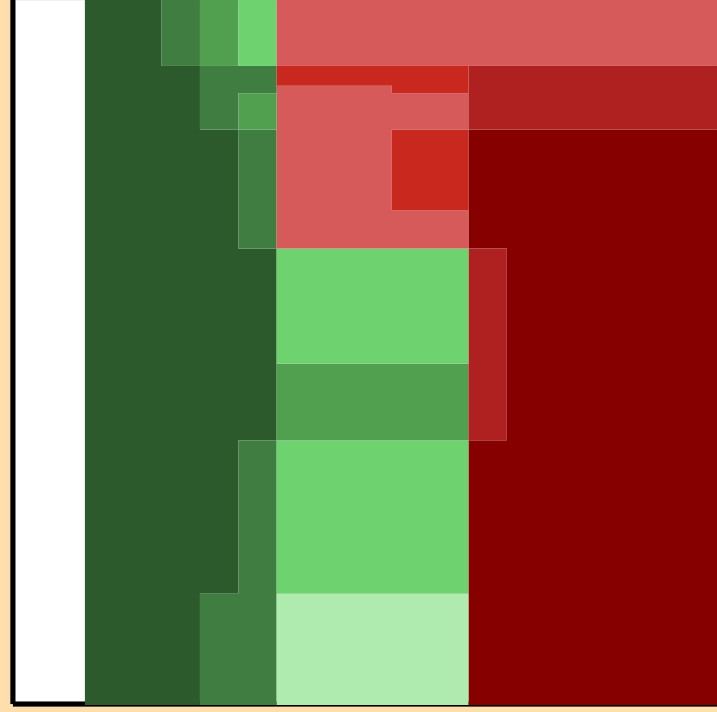
\Delta\sigma/\sigma vs. E for ^{244}\text{Am}(n,p)
