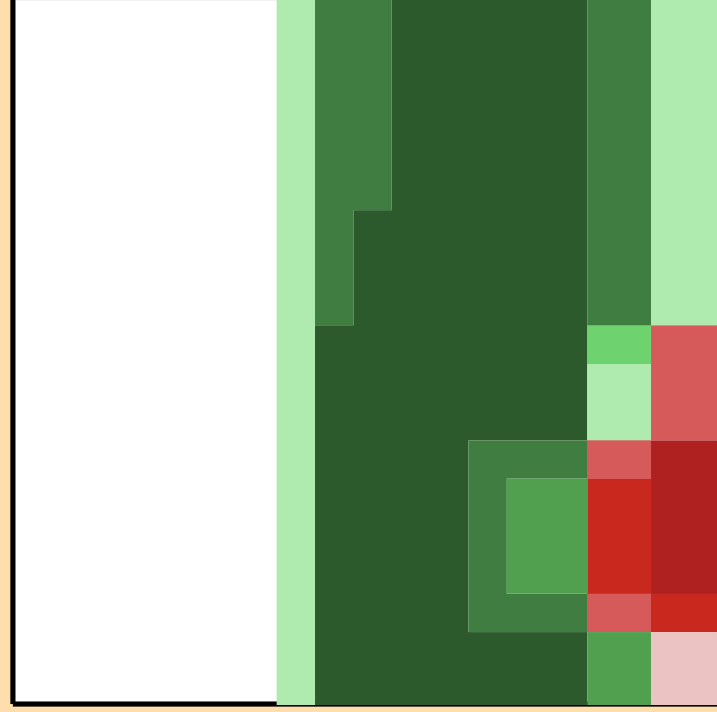
\Delta\sigma/\sigma vs. E for ^{244}\text{Am}(n,2n)
