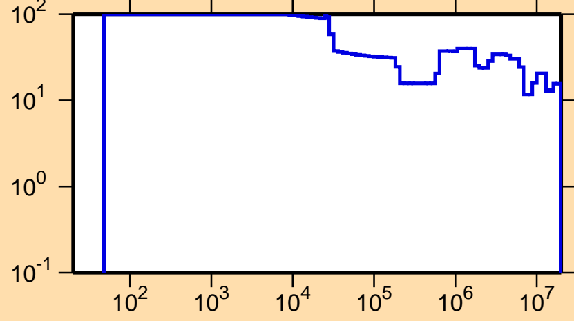
\Delta\sigma/\sigma vs. E for ^{244}\text{Am}(n,\text{el.})
