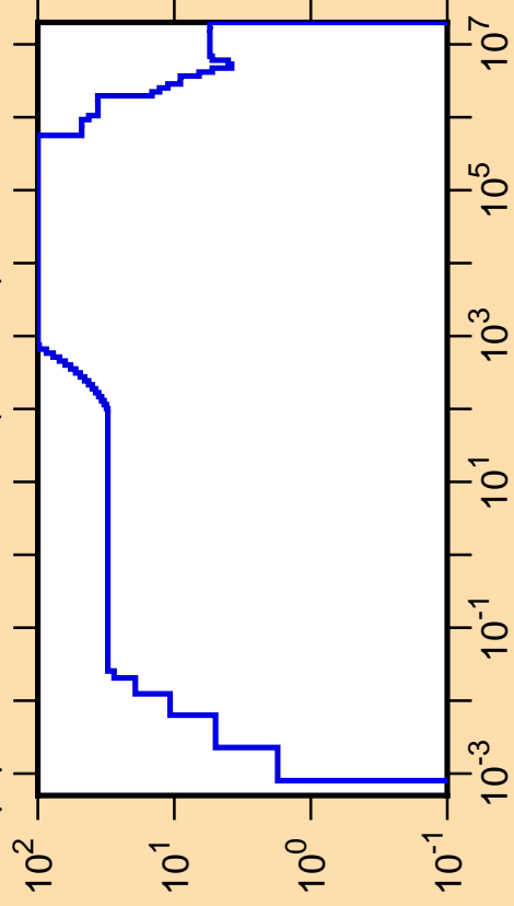
\Delta\mu/\mu vs. E for ^{245}\text{Am}(\text{mt251})
