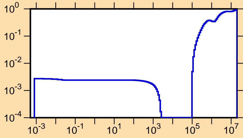
\mu vs. E for ^{245}\text{Am}(\text{mt251})
