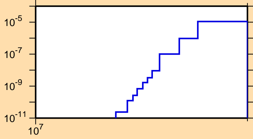
\sigma vs. E for ^{245}\text{Am}(n,nt)
