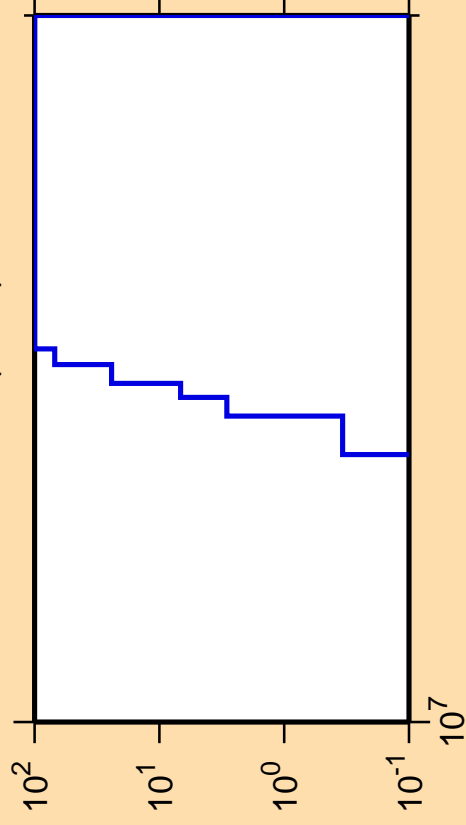
\Delta\sigma/\sigma vs. E for ^{245}\text{Am}(n,nd)
