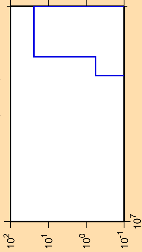
\Delta\sigma/\sigma vs. E for ^{245}\text{Am}(n,\text{He3})
