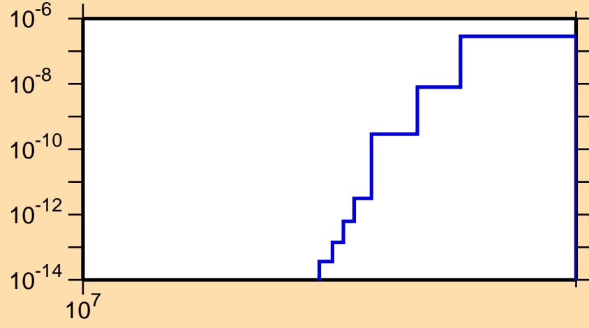
\sigma vs. E for ^{245}\text{Am}(n,2np)
