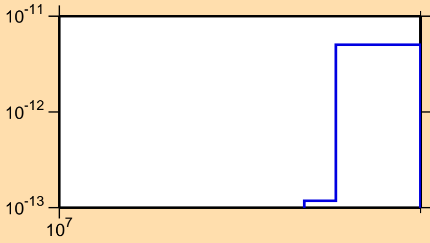
\sigma vs. E for ^{245}\text{Am}(n,\text{He3})
