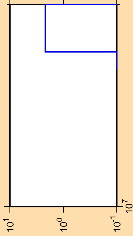
\Delta\sigma/\sigma vs. E for ^{245}\text{Am}(\text{mt } 11)
