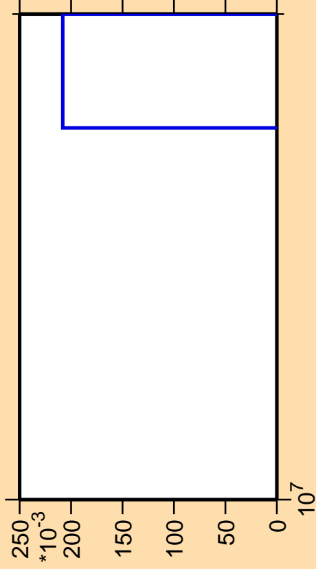
\Delta\sigma/\sigma vs. E for ^{245}\text{Am} (mt 42)
