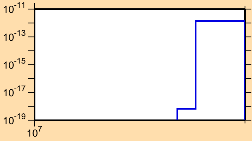
\sigma vs. E for ^{245}\text{Am}(\text{mt } 11)
