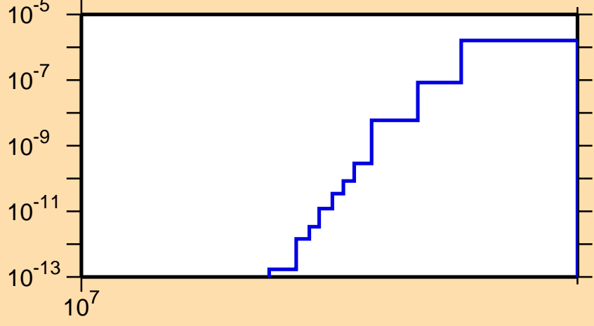
\sigma vs. E for ^{245}\text{Am}(n,nd)
