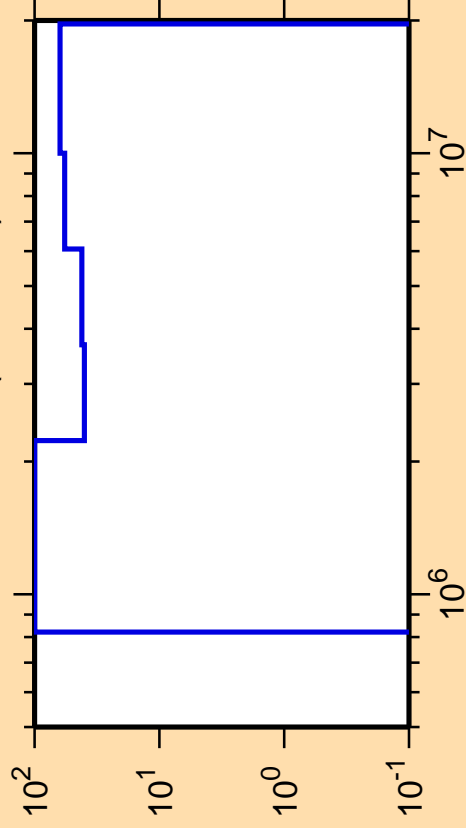
\Delta\sigma/\sigma vs. E for ^{245}\text{Am}(n,\text{ncont.})
