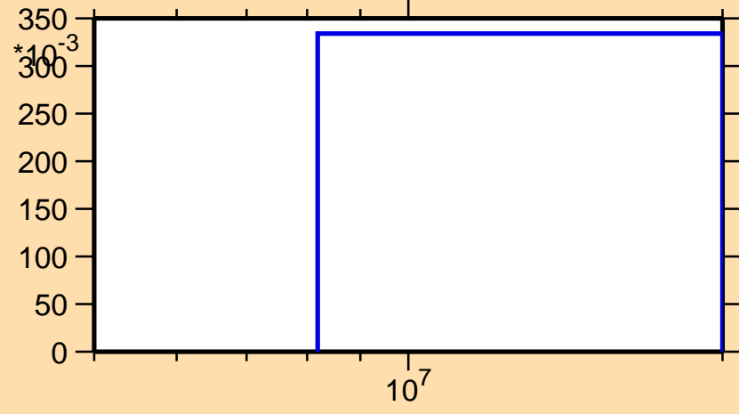
\sigma vs. E for ^{245}\text{Am}(n,3n)
