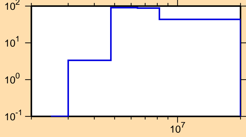
\Delta\sigma/\sigma vs. E for ^{245}\text{Am}(n,p)
