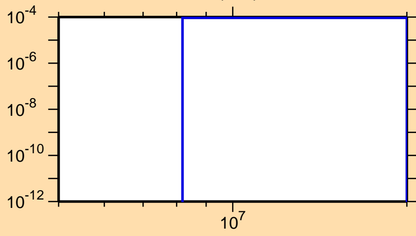
\sigma vs. E for ^{245}\text{Am}(n,d)
