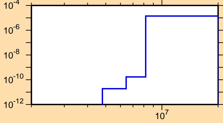
\sigma vs. E for ^{245}\text{Am}(n,n\alpha)
