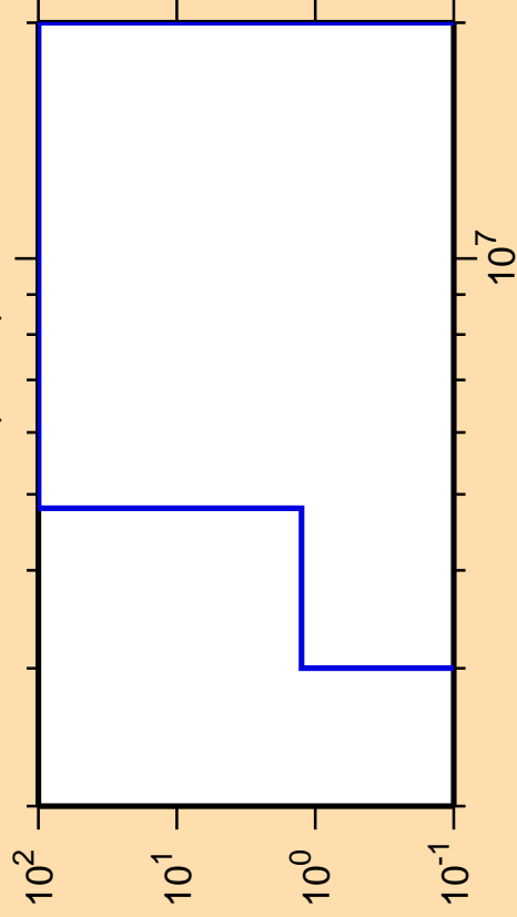
\Delta\sigma/\sigma vs. E for ^{245}\text{Am}(n,n\alpha)
