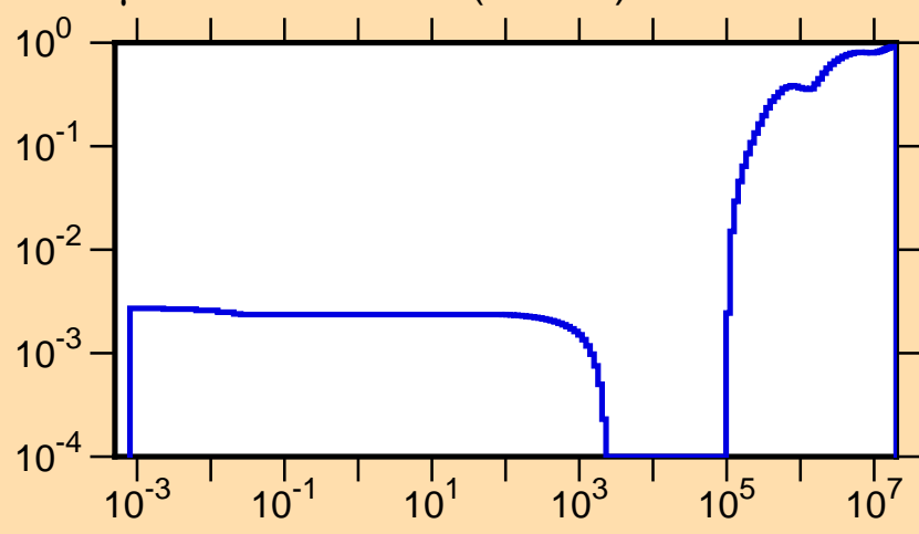
\mu vs. E for ^{246}\text{Am}(\text{mt251})
