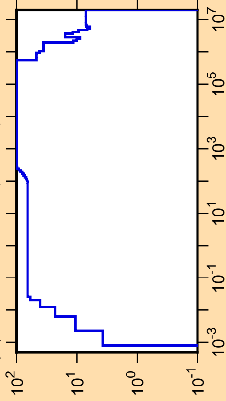
\Delta\mu/\mu vs. E for ^{246}\text{Am}(\text{mt251})
