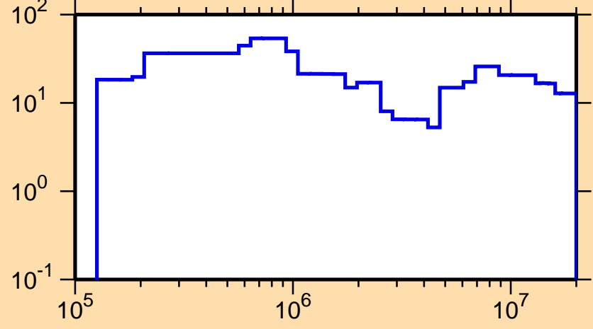
\Delta\sigma/\sigma vs. E for ^{246}\text{Am}(n,\text{el.})
