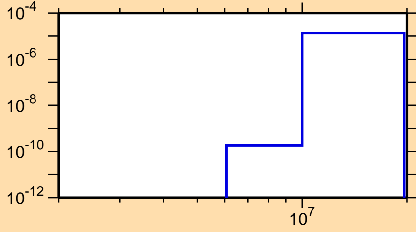
\sigma vs. E for ^{246}\text{Am}(n,n\alpha)
