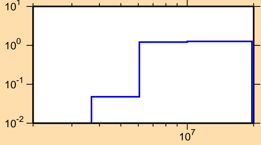
\sigma vs. E for ^{246}\text{Am}(n,2n)
