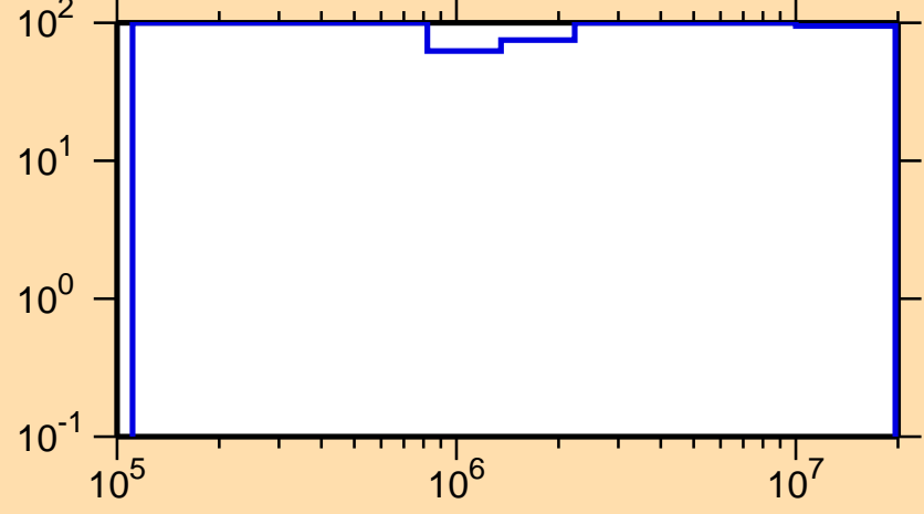
\Delta\sigma/\sigma vs. E for ^{246}\text{Am}(n,f)
