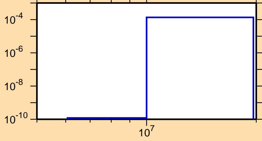
\sigma vs. E for ^{246}\text{Am}(n,d)
