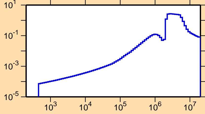
\sigma vs. E for ^{246}\text{Am}(n,\text{inel.})
