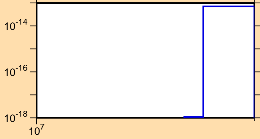
\sigma vs. E for ^{246}\text{Am} (mt 42)
