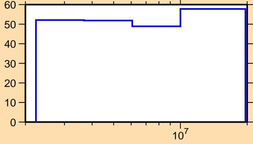
\Delta\sigma/\sigma vs. E for ^{246}\text{Am}(n,ncont.)
