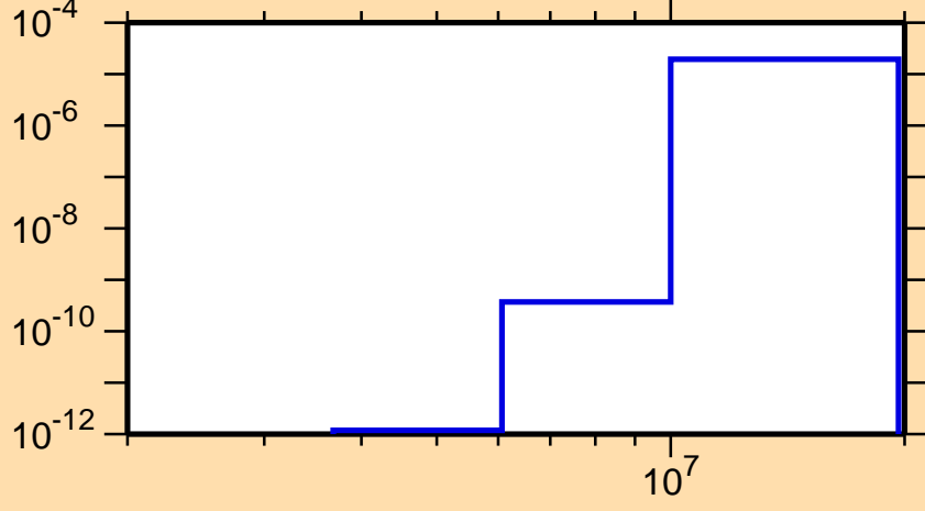
\sigma vs. E for ^{246}\text{Am}(n,\alpha)
