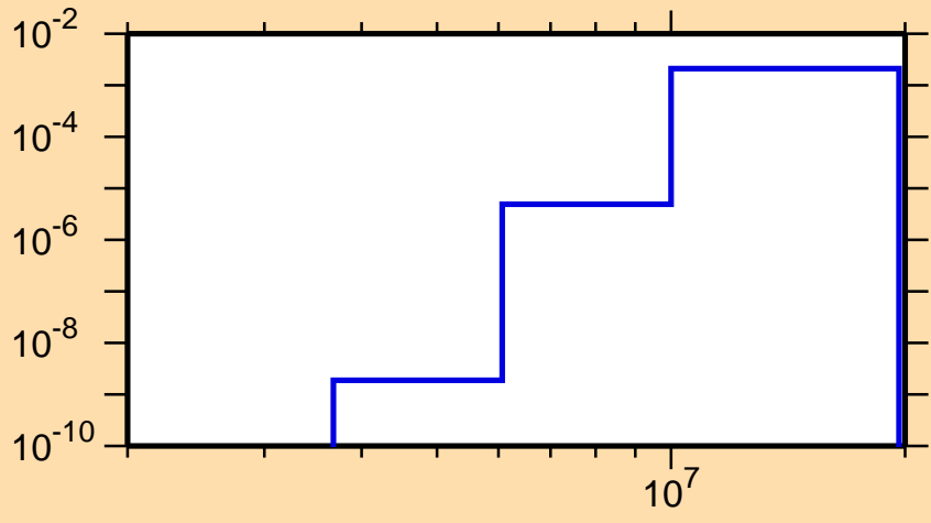
\sigma vs. E for ^{246}\text{Am}(n,p)
