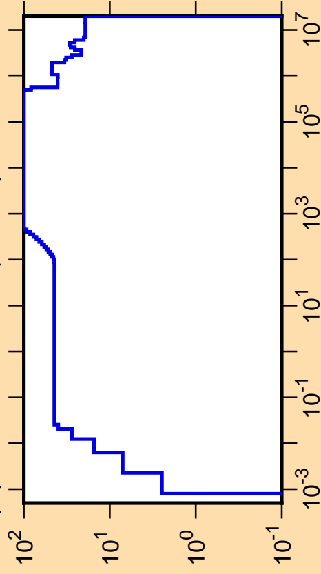
\Delta\mu/\mu vs. E for ^{247}\text{Am}(\text{mt251})
