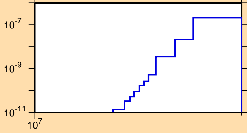
\sigma vs. E for ^{247}\text{Am}(n,2n\alpha)
