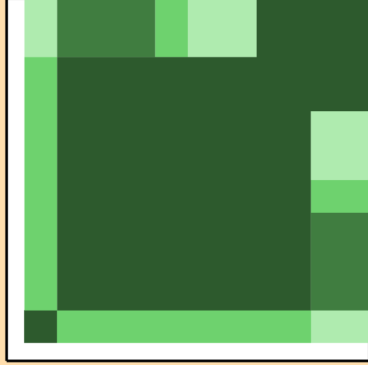
\sigma vs. E for ^{247}\text{Am}(n,2n)
