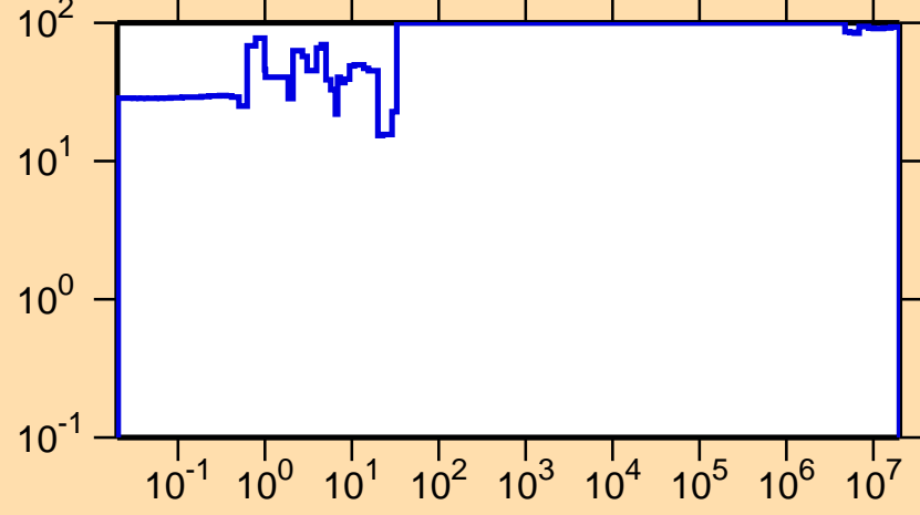
\Delta\sigma/\sigma vs. E for ^{247}\text{Am}(n,f)
