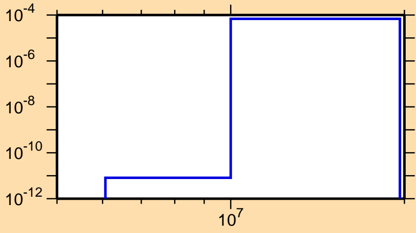
\sigma vs. E for ^{247}\text{Am}(n,np)
