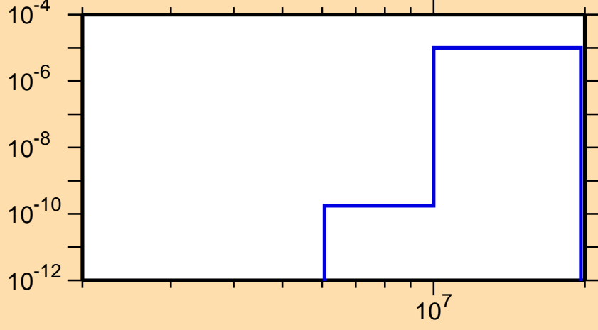
\sigma vs. E for ^{247}\text{Am}(n,n\alpha)
