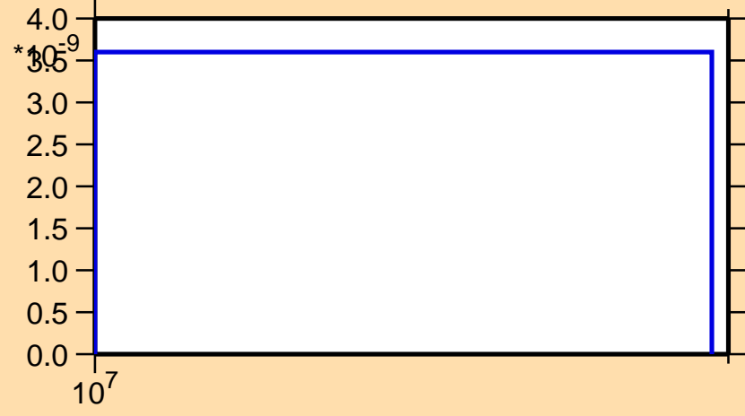
\sigma vs. E for ^{247}\text{Am}(n,2n\alpha)
