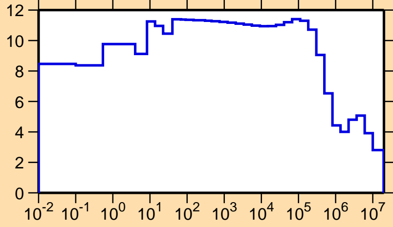
\sigma vs. E for ^{247}\text{Am}(n,\text{el.})
