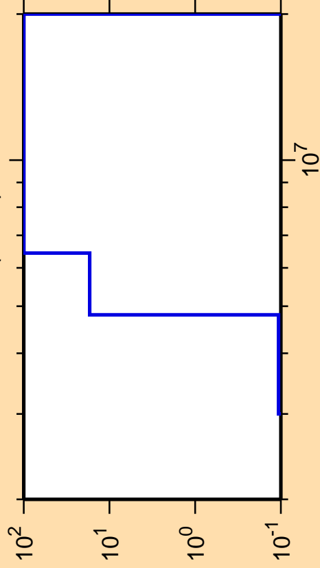
\Delta\sigma/\sigma vs. E for ^{247}\text{Am}(n,n\alpha)
