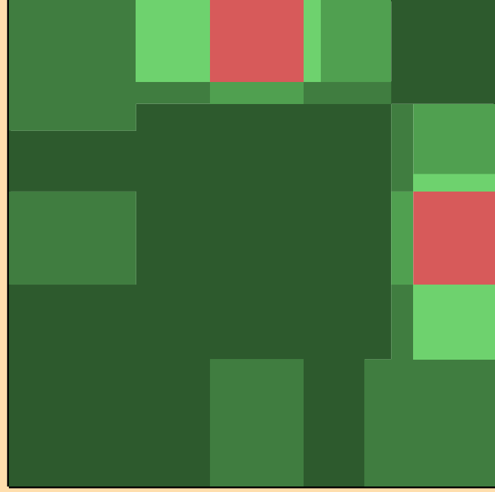
\sigma vs. E for ^{247}\text{Am}(n,n\text{cont.})
