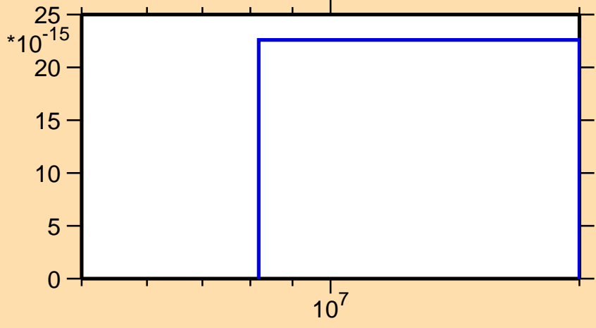
\sigma vs. E for ^{247}\text{Am}(\text{mt } 11)
