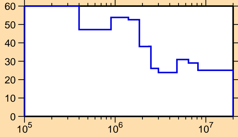
\Delta\sigma/\sigma vs. E for ^{247}\text{Am}(n,n\text{onel.})
