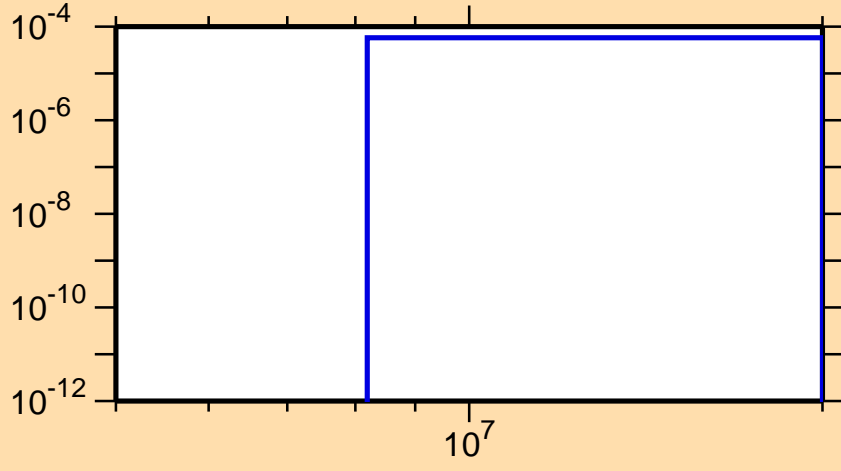
\sigma vs. E for ^{247}\text{Am}(n,d)
