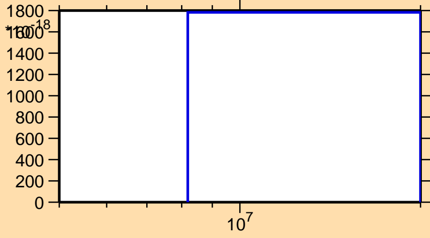
\sigma vs. E for ^{247}\text{Am} (mt 42)
