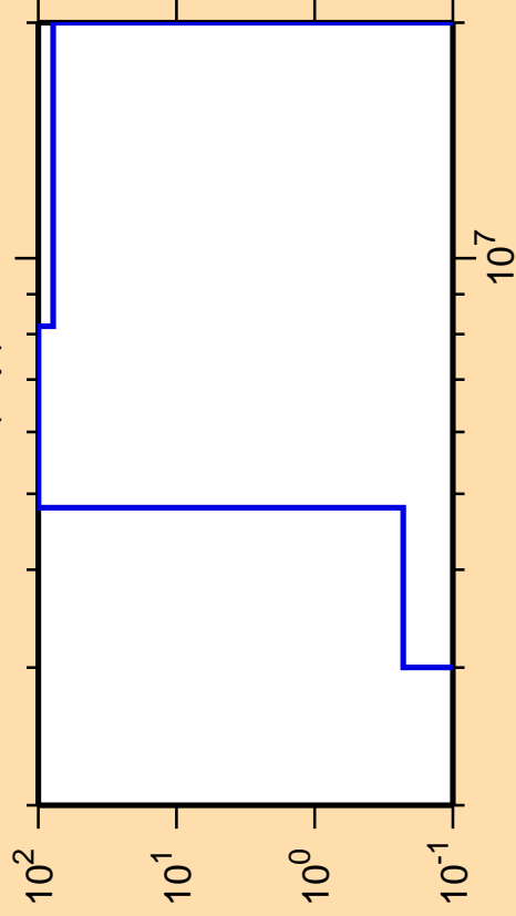
\Delta\sigma/\sigma vs. E for ^{247}\text{Am}(n,p)
