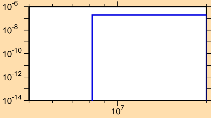
\sigma vs. E for ^{247}\text{Am}(n,nt)
