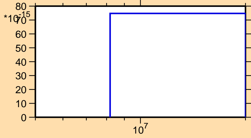
\sigma vs. E for ^{247}\text{Am}(n,3n\alpha)
