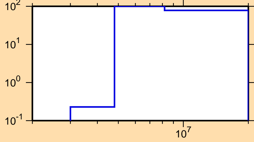
\Delta\sigma/\sigma vs. E for ^{247}\text{Am}(n,p)
