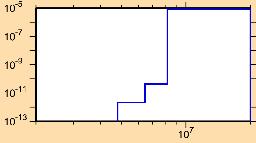
\sigma vs. E for ^{247}\text{Am}(n,n\alpha)
