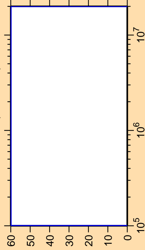
\Delta\sigma/\sigma vs. E for ^{247}\text{Am}(n,\text{ncont.})
