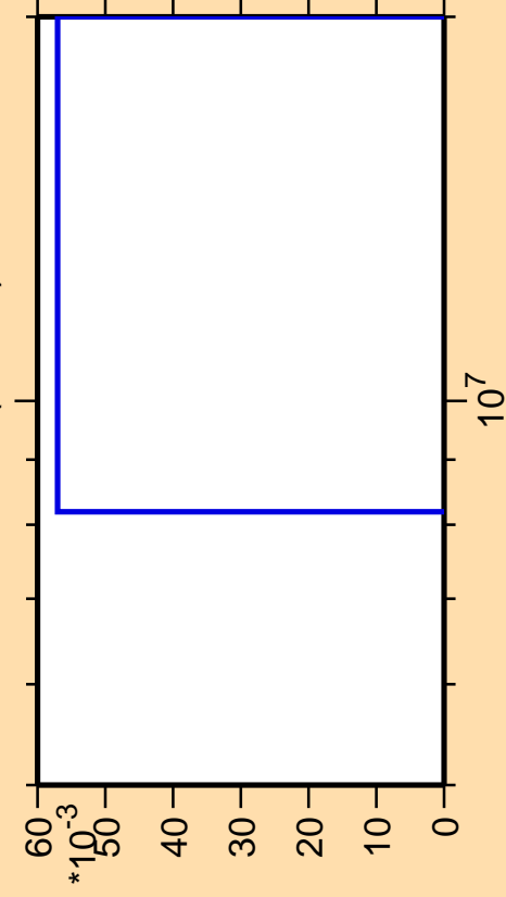
\Delta\sigma/\sigma vs. E for ^{247}\text{Am}(\text{mt } 11)
