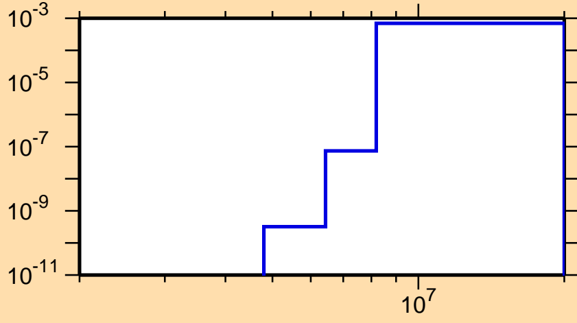
\sigma vs. E for ^{247}\text{Am}(n,p)
