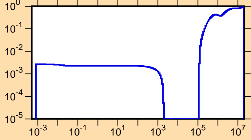
\mu vs. E for ^{248}\text{Am}(\text{mt251})
