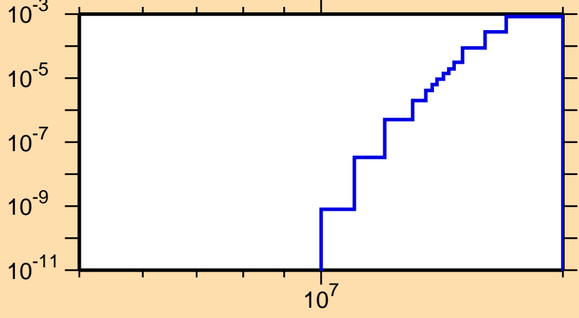
\sigma vs. E for ^{248}\text{Am}(n,np)
