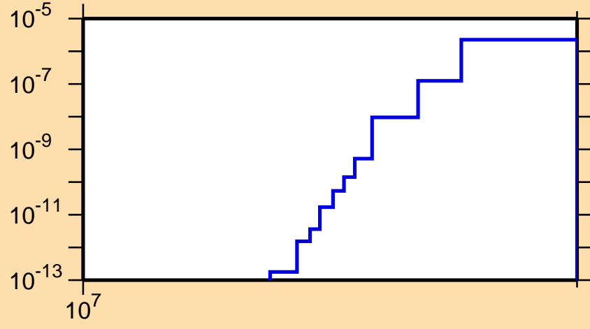
\sigma vs. E for ^{248}\text{Am}(n,2np)
