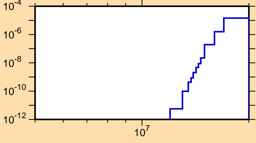
\sigma vs. E for ^{248}\text{Am}(n,\text{nd})
