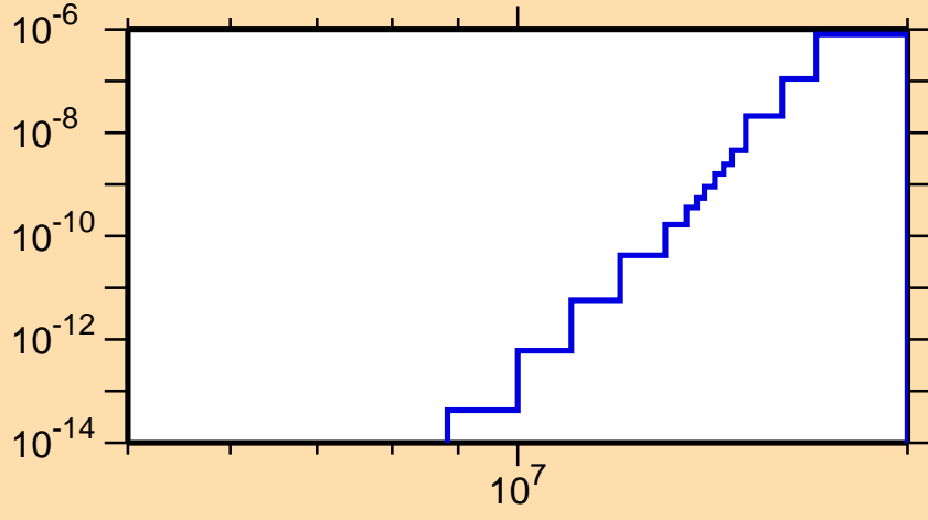
\sigma vs. E for ^{248}\text{Am}(n,2n\alpha)
