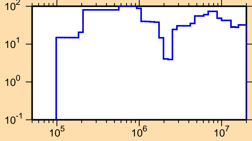
\Delta\sigma/\sigma vs. E for ^{248}\text{Am}(n,\text{el.})
