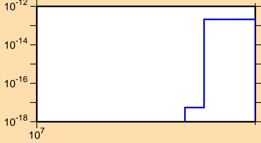
\sigma vs. E for ^{248}\text{Am} (mt 42)
