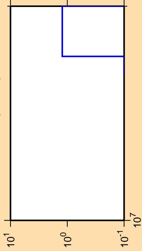
\Delta\sigma/\sigma vs. E for ^{248}\text{Am}(n,\text{He3})
