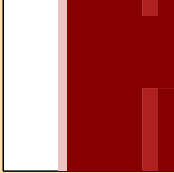
\Delta\sigma/\sigma vs. E for ^{248}\text{Am}(n,2n)
