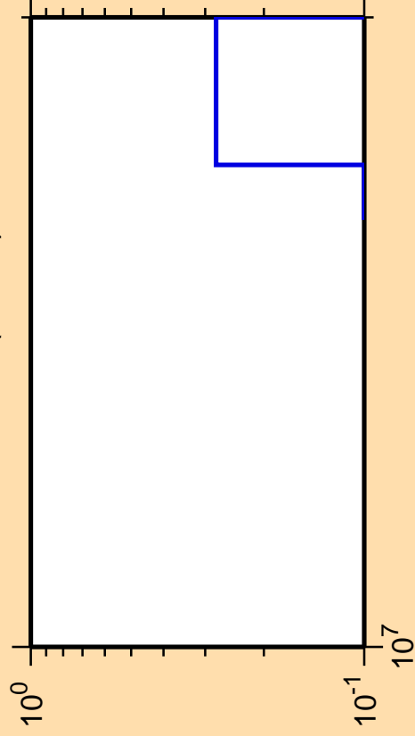
\Delta\sigma/\sigma vs. E for ^{248}\text{Am} (mt 42)
