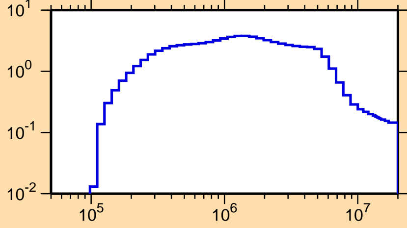
\sigma vs. E for ^{248}\text{Am}(n,\text{inel.})
