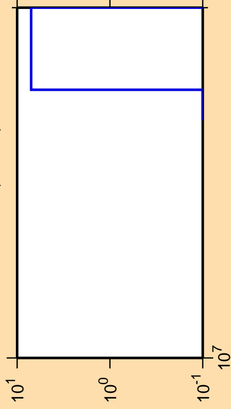
\Delta\sigma/\sigma vs. E for ^{248}\text{Am}(\text{mt } 11)
