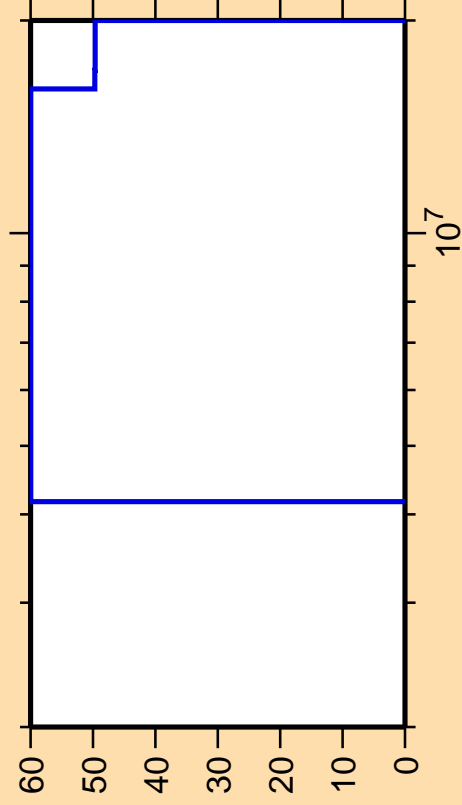
\Delta\sigma/\sigma vs. E for ^{248}\text{Am}(n,f)
