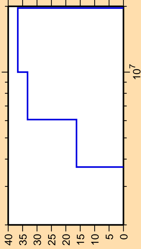
\Delta\sigma/\sigma vs. E for ^{248}\text{Am}(n,n\text{cont.})
