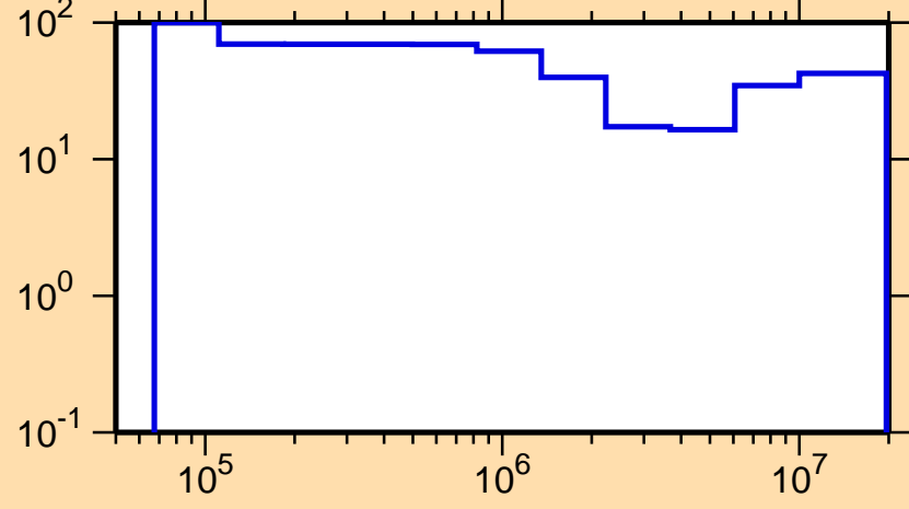
\Delta\sigma/\sigma vs. E for ^{248}\text{Am}(n,inel.)
