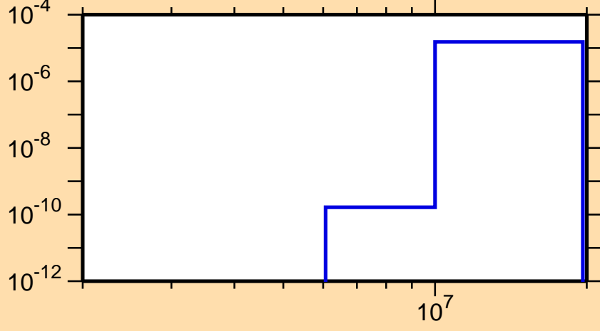
\sigma vs. E for ^{248}\text{Am}(n,n\alpha)
