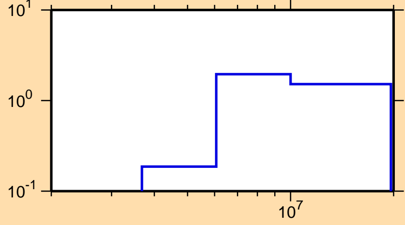
\sigma vs. E for ^{248}\text{Am}(n,2n)
