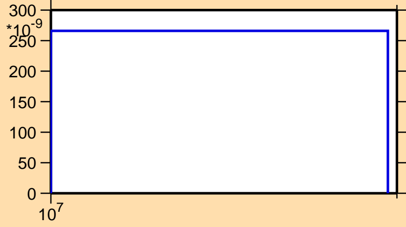
\sigma vs. E for ^{248}\text{Am}(n,nt)
