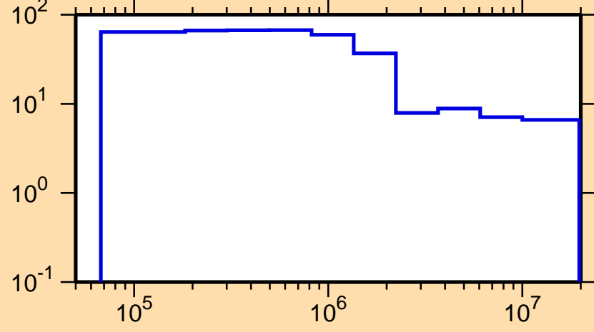
\Delta\sigma/\sigma vs. E for ^{248}\text{Am}(n,\text{nonel.})
