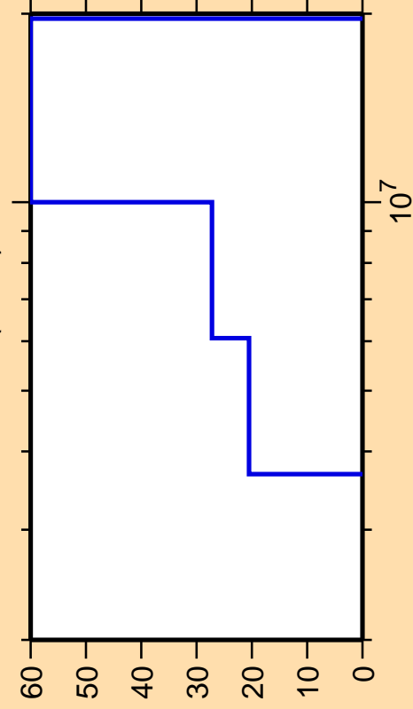
\Delta\sigma/\sigma vs. E for ^{248}\text{Am}(n,2n)
