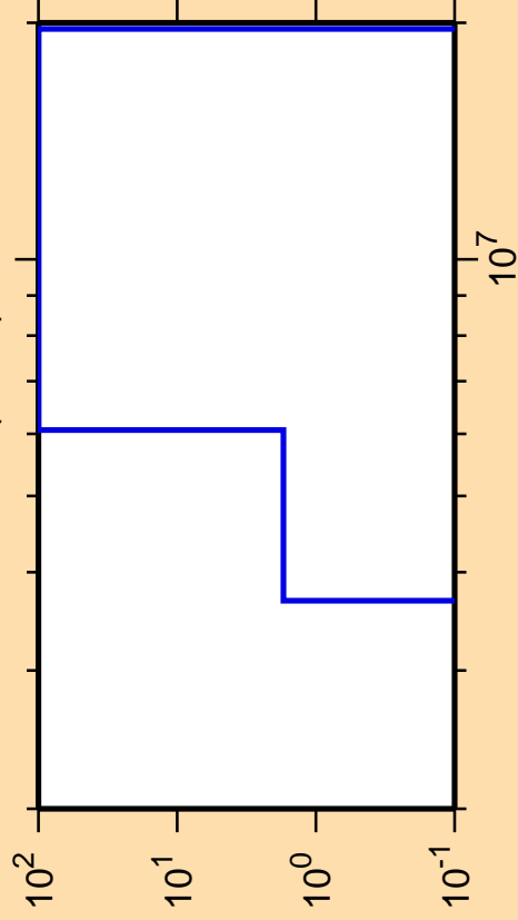
\Delta\sigma/\sigma vs. E for ^{248}\text{Am}(n,n\alpha)
