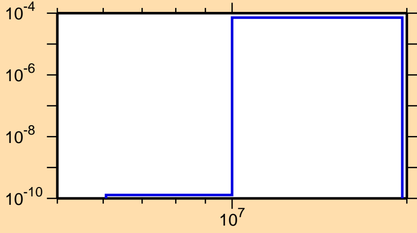
\sigma vs. E for ^{248}\text{Am}(n,t)
