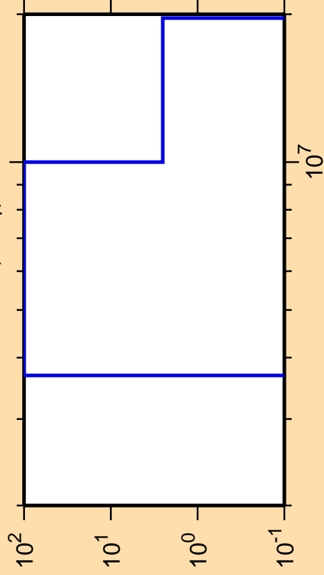
\Delta\sigma/\sigma vs. E for ^{248}\text{Am}(n,n_1)
