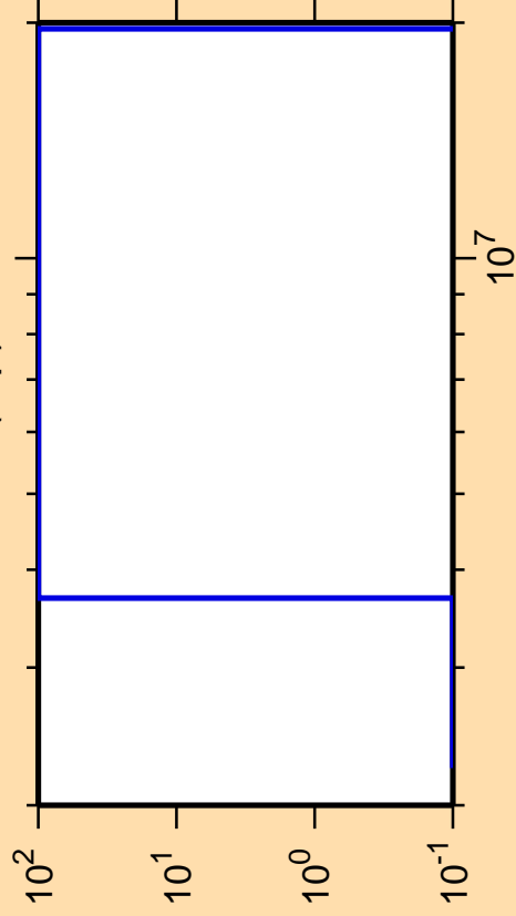
\Delta\sigma/\sigma vs. E for ^{248}\text{Am}(n,p)
