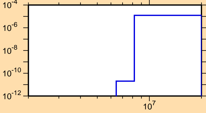
\sigma vs. E for ^{248}\text{Am}(n,\alpha)
