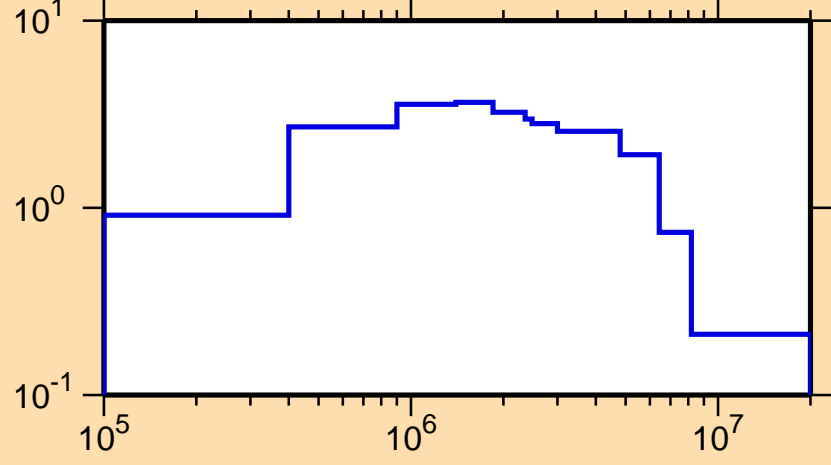
\sigma vs. E for ^{248}\text{Am}(n,n\text{cont.})
