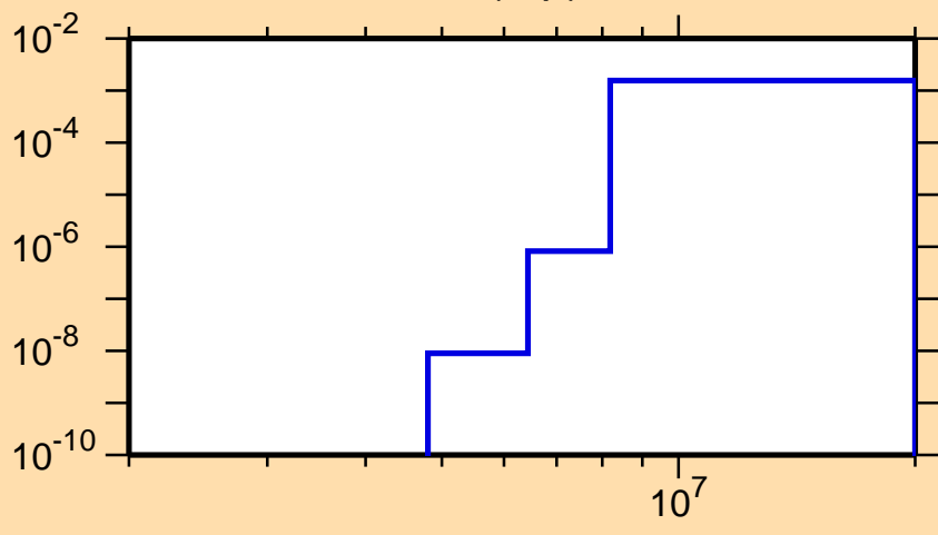
\sigma vs. E for ^{248}\text{Am}(n,p)
