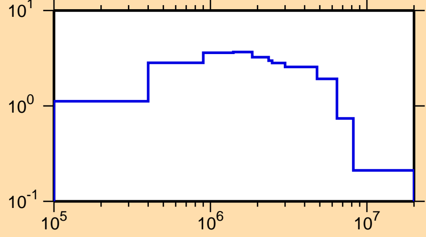
\sigma vs. E for ^{248}\text{Am}(n,\text{inel.})
