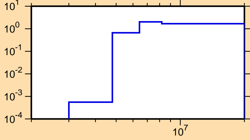
\sigma vs. E for ^{248}\text{Am}(n,2n)
