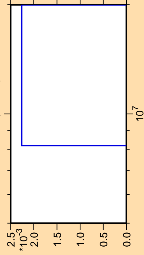
\Delta\sigma/\sigma vs. E for ^{248}\text{Am}(\text{mt } 42)
