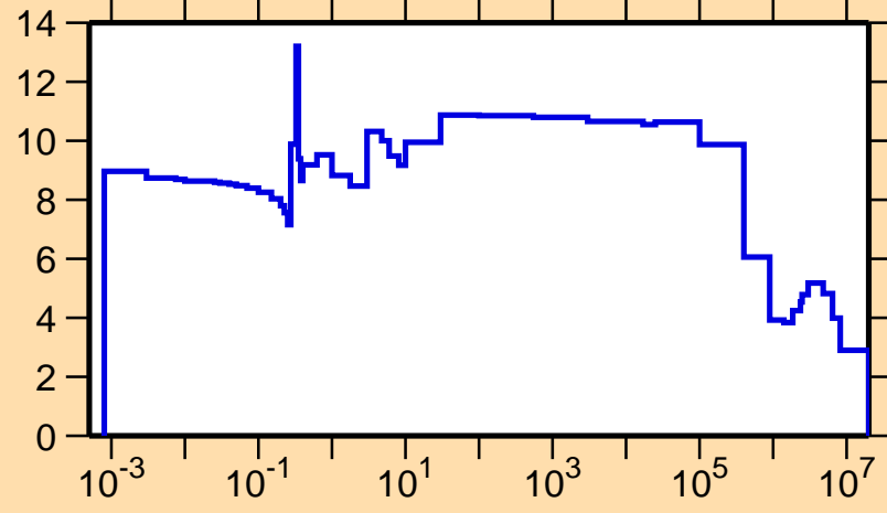
\sigma vs. E for ^{248}\text{Am}(n,\text{el.})
