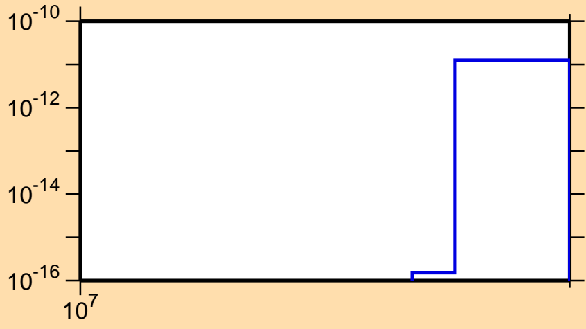
\sigma vs. E for ^{249}\text{Am}(\text{mt } 11)
