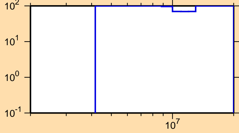
\Delta\sigma/\sigma vs. E for ^{249}\text{Am}(n,\gamma)
