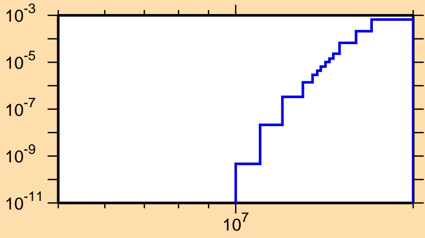
\sigma vs. E for ^{249}\text{Am}(n,np)
