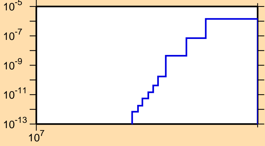
\sigma vs. E for ^{249}\text{Am}(n,nd)
