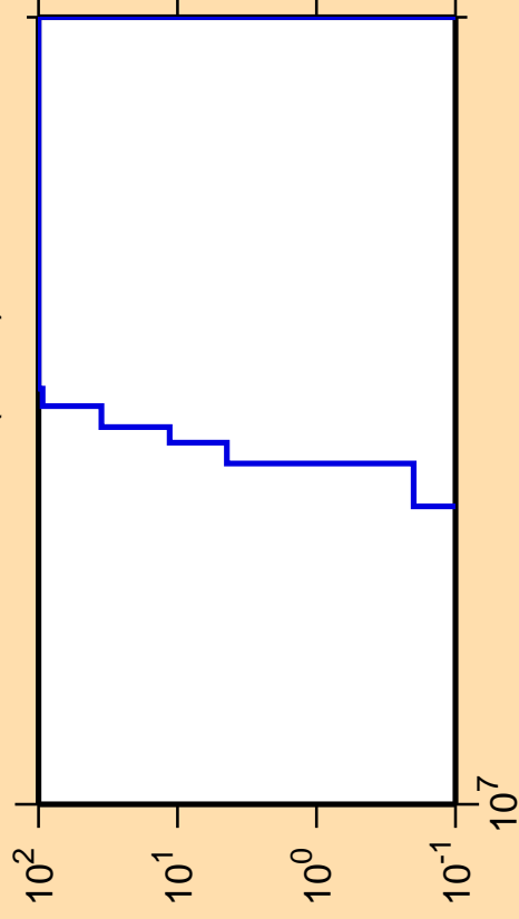
\Delta\sigma/\sigma vs. E for ^{249}\text{Am}(n,nd)
