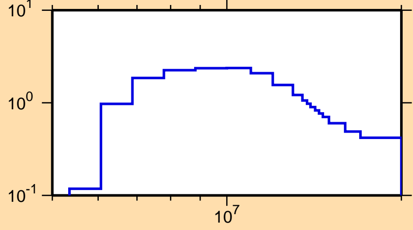
\sigma vs. E for ^{249}\text{Am}(n,2n)
