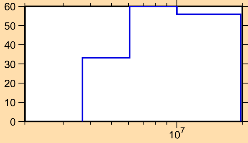
\Delta\sigma/\sigma vs. E for ^{249}\text{Am}(n,ncont.)
