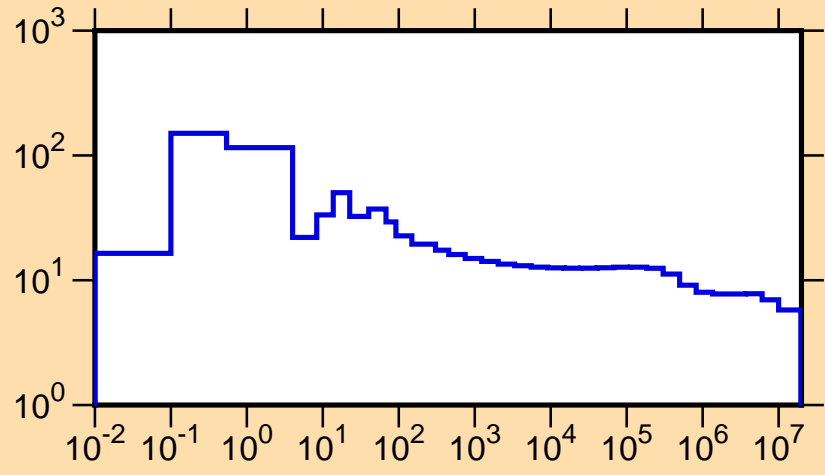
\sigma vs. E for ^{249}\text{Am}(n,\text{tot.})
