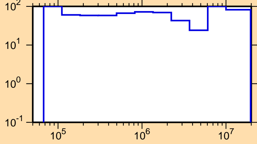
\Delta\sigma/\sigma vs. E for ^{249}\text{Am}(n,\text{inel.})
