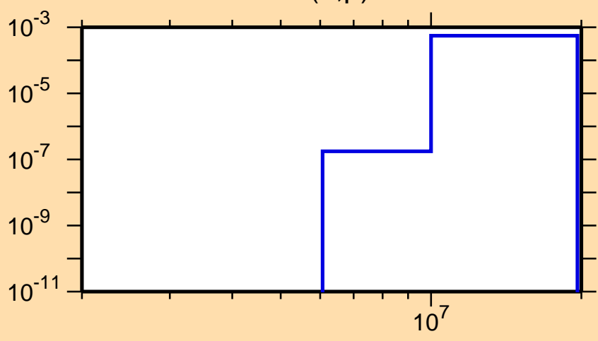
\sigma vs. E for ^{249}\text{Am}(n,p)
