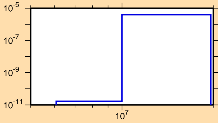
\sigma vs. E for ^{249}\text{Am}(n,n\alpha)
