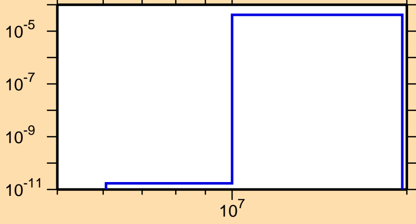
\sigma vs. E for ^{249}\text{Am}(n,d)
