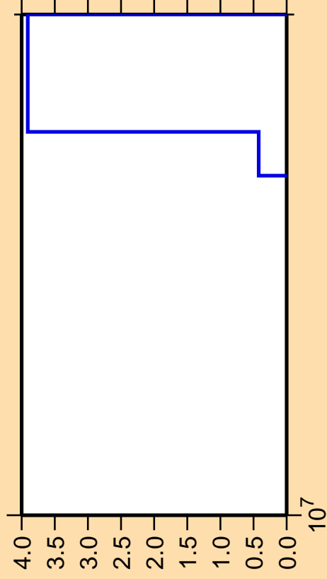
\Delta\sigma/\sigma vs. E for ^{234}\text{Bk}(n,\text{pd})
