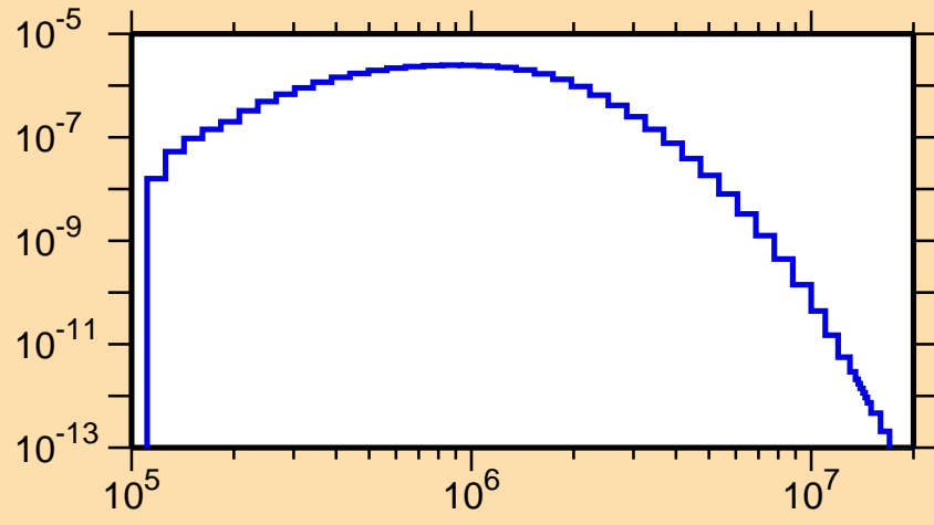
\sigma vs. E for ^{234}\text{Bk}(n,n_1)
