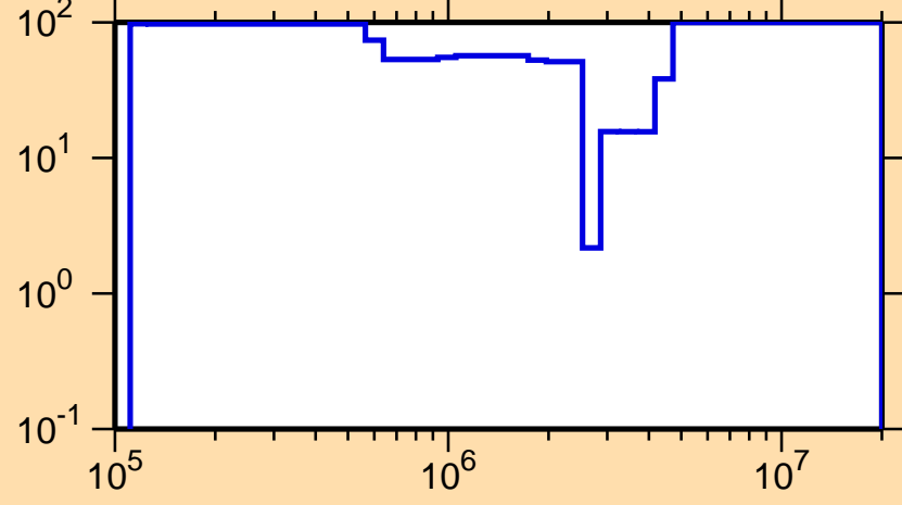
\Delta\sigma/\sigma vs. E for ^{234}\text{Bk}(n,n\text{cont.})
