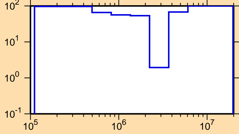
\Delta\sigma/\sigma vs. E for ^{234}\text{Bk}(n,\text{inel.})
