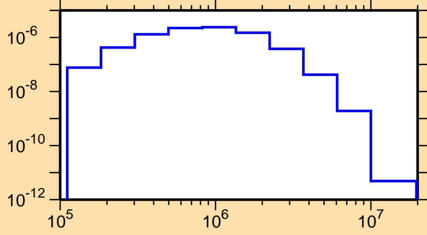
\sigma vs. E for ^{234}\text{Bk}(n,n_1)
