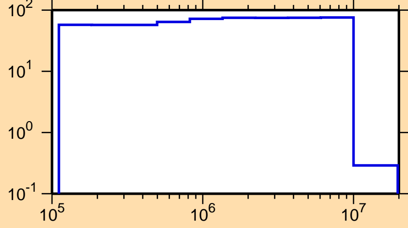
\Delta\sigma/\sigma vs. E for ^{234}\text{Bk}(n,n_1)
