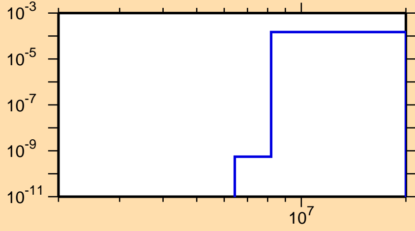
\sigma vs. E for ^{234}\text{Bk}(n,t)
