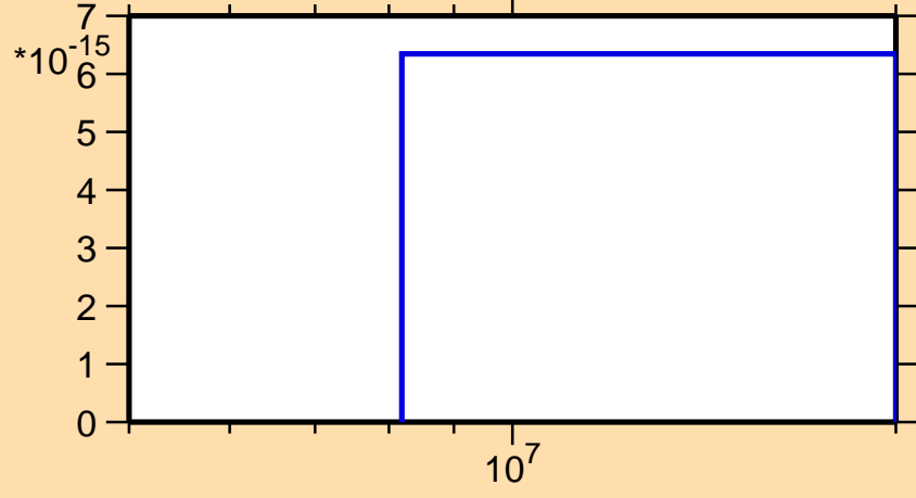
\sigma vs. E for ^{234}\text{Bk}(n,\text{pd})
