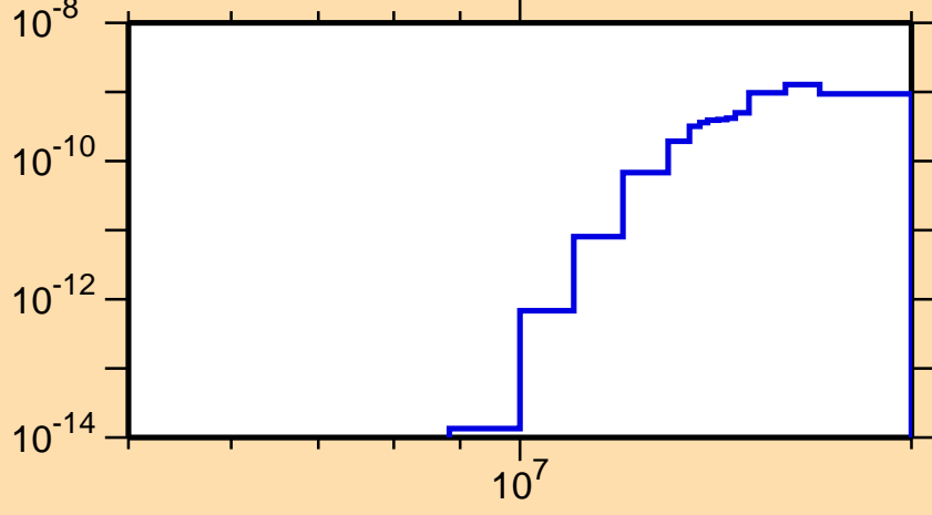
\sigma vs. E for ^{235}\text{Bk}(n,2n\alpha)
