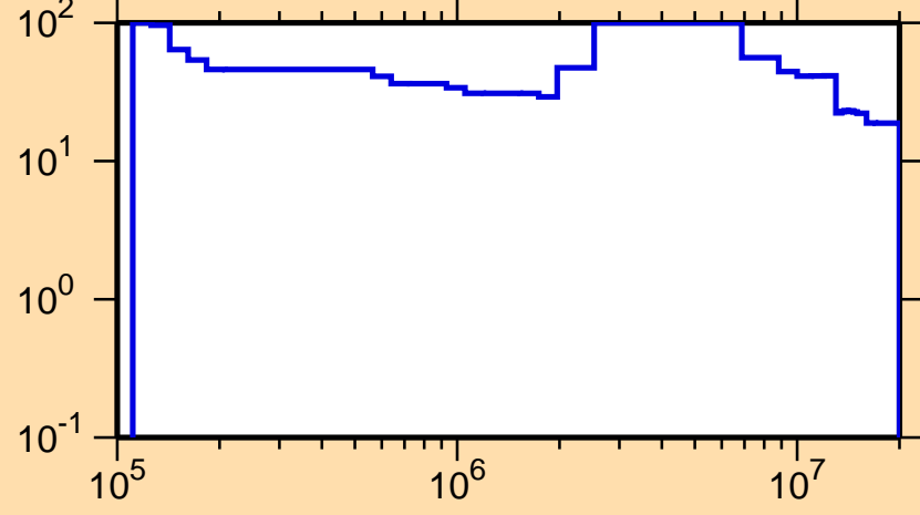
\Delta\sigma/\sigma vs. E for ^{235}\text{Bk}(n,\text{inel.})
