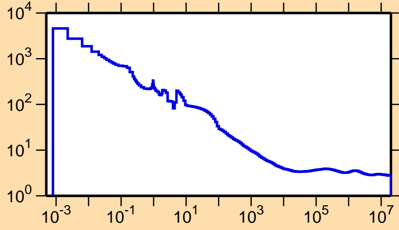
\sigma vs. E for ^{235}\text{Bk}(n,f)
