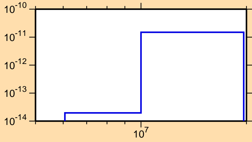
\sigma vs. E for ^{235}\text{Bk}(n,p\alpha)
