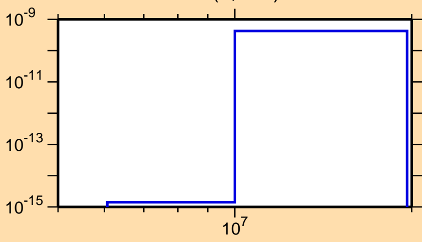
\sigma vs. E for ^{235}\text{Bk}(n,2n\alpha)
