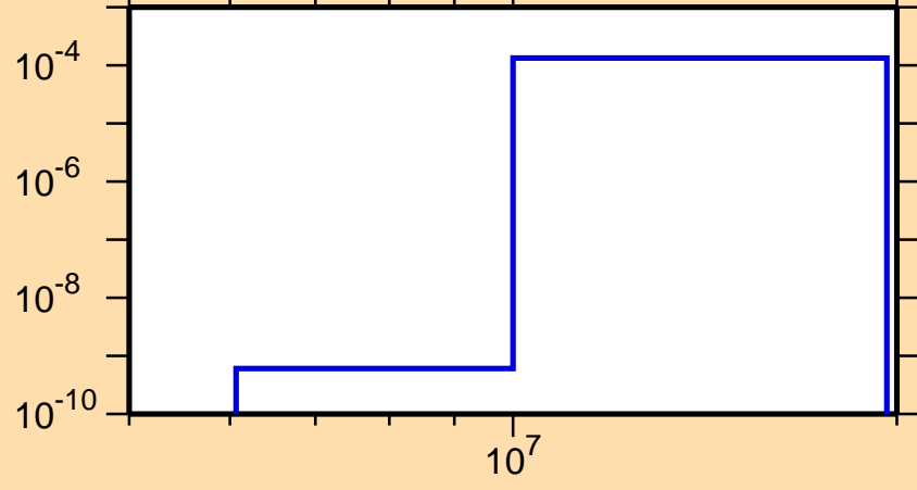
\sigma vs. E for ^{235}\text{Bk}(n,t)
