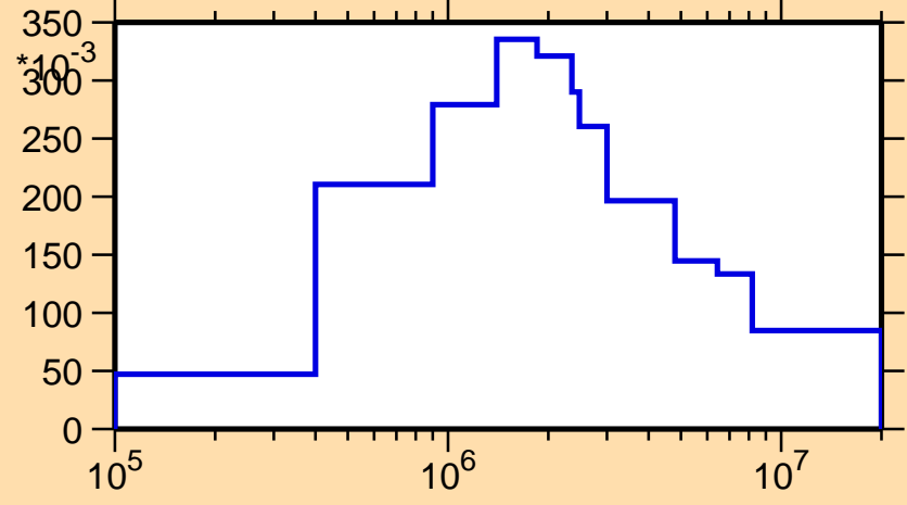
\sigma vs. E for ^{235}\text{Bk}(n,\text{inel.})
