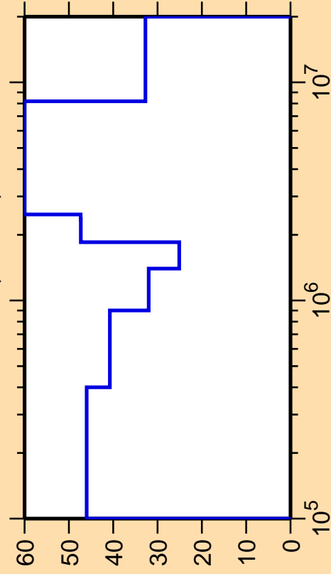
\Delta\sigma/\sigma vs. E for ^{235}\text{Bk}(n,\text{inel.})
