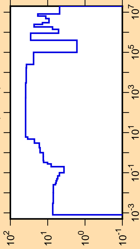
\Delta\sigma/\sigma vs. E for ^{235}\text{Bk}(n,\text{tot.})
