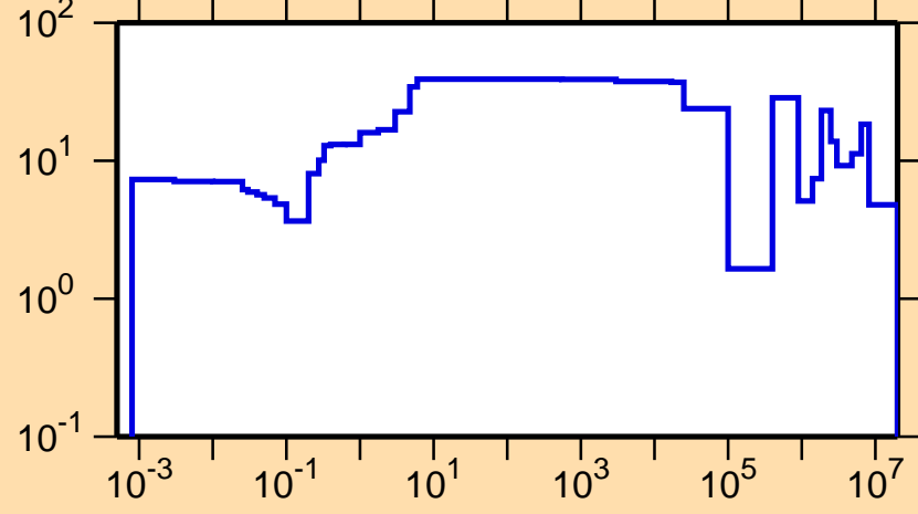
\Delta\sigma/\sigma vs. E for ^{235}\text{Bk}(n,\text{tot.})
