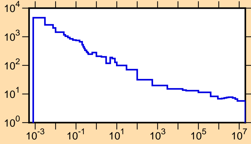
\sigma vs. E for ^{235}\text{Bk}(n,\text{tot.})
