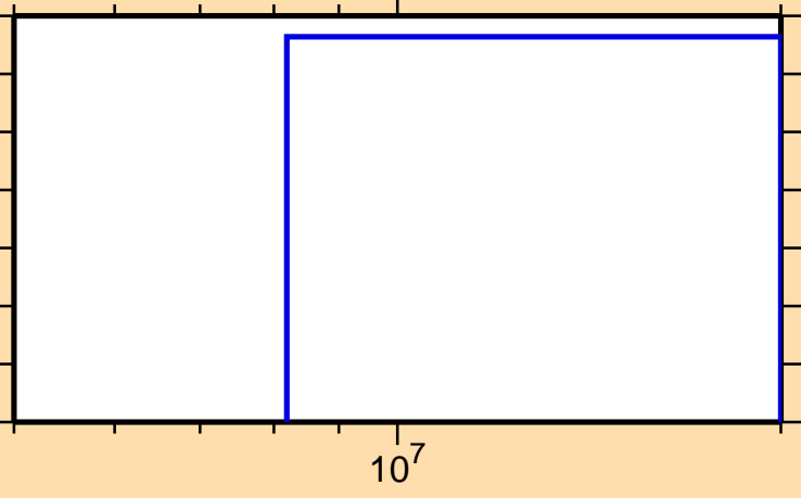
\sigma vs. E for ^{235}\text{Bk}(n,3n)
