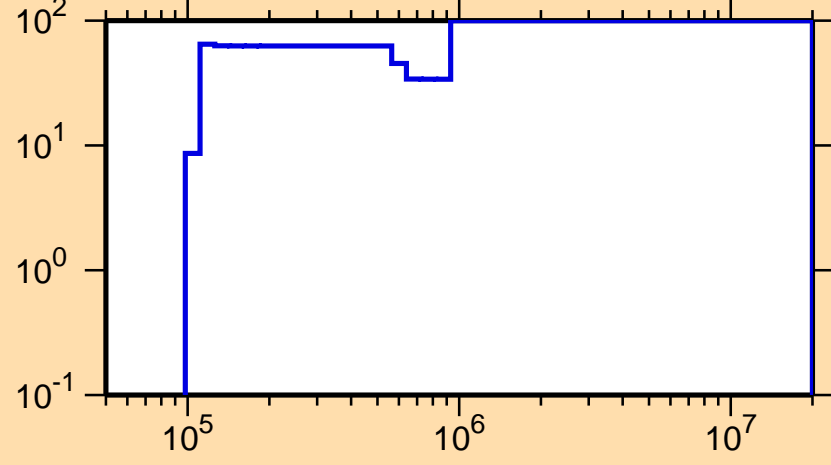
\Delta\sigma/\sigma vs. E for ^{236}\text{Bk}(n,n_1)
