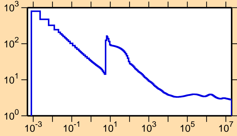
\sigma vs. E for ^{236}\text{Bk}(n,f)
