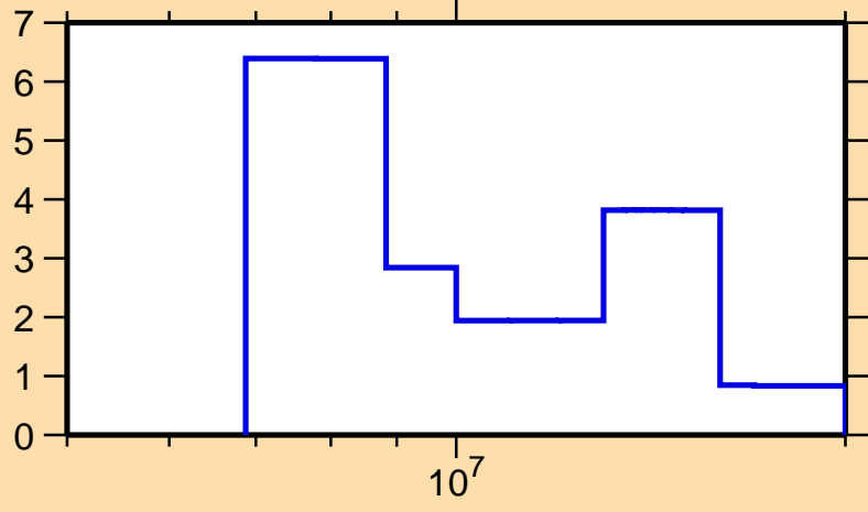
\Delta\sigma/\sigma vs. E for ^{236}\text{Bk}(n,\text{nonel.})
