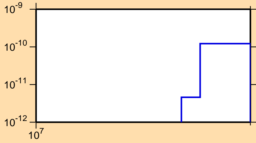
\sigma vs. E for ^{236}\text{Bk}(n,nt)
