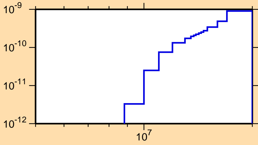
\sigma vs. E for ^{236}\text{Bk}(n,2n\alpha)
