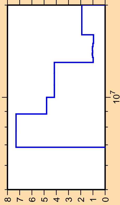
\Delta\sigma/\sigma vs. E for ^{236}\text{Bk}(n,f)
