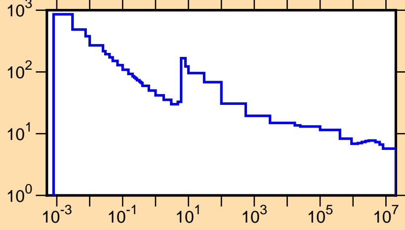
\sigma vs. E for ^{236}\text{Bk}(n,\text{tot.})
