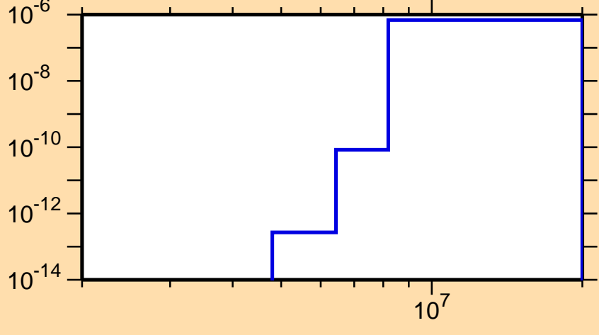
\sigma vs. E for ^{236}\text{Bk}(n,t)
