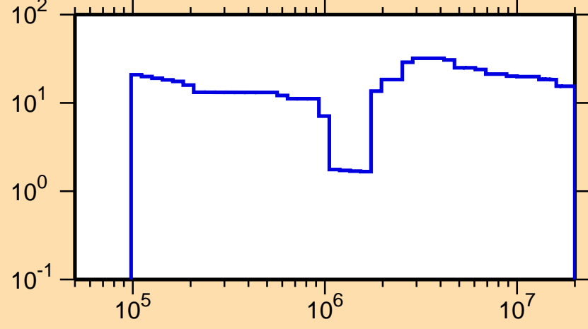
\Delta\sigma/\sigma vs. E for ^{237}\text{Bk}(n,\text{nonel.})
