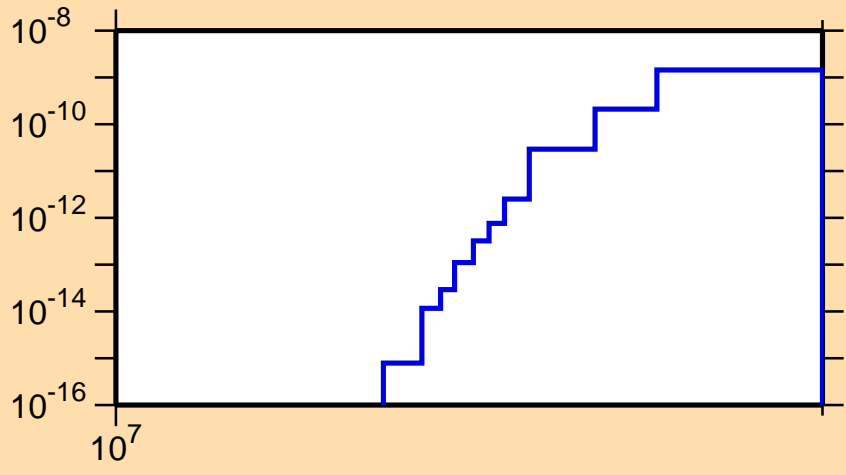
\sigma vs. E for ^{237}\text{Bk}(n,2np)
