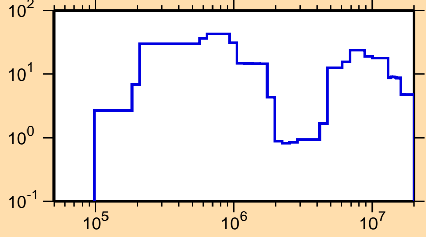
\Delta\sigma/\sigma vs. E for ^{237}\text{Bk}(n,\text{tot.})
