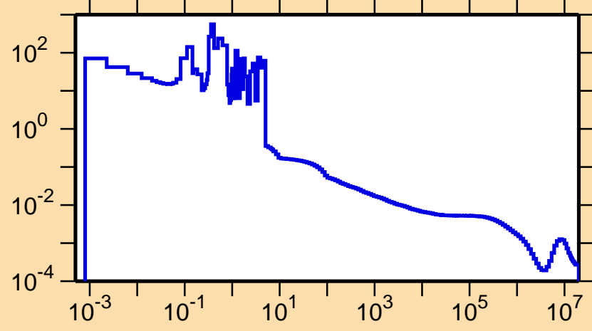
\sigma vs. E for ^{237}\text{Bk}(n,\gamma)
