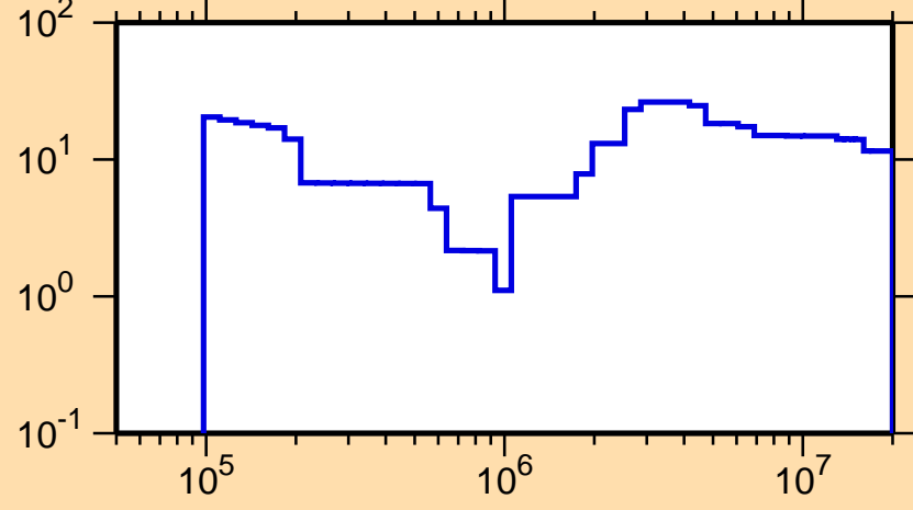
\Delta\sigma/\sigma vs. E for ^{237}\text{Bk}(n,f)
