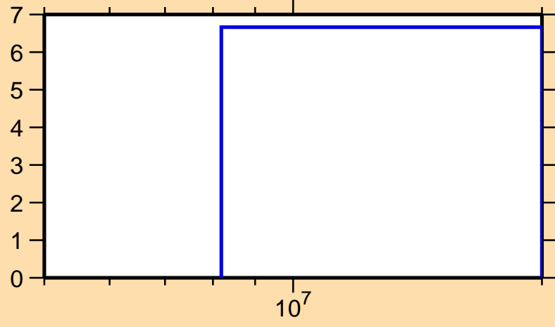
\Delta\sigma/\sigma vs. E for ^{237}\text{Bk}(n,\text{el.})
