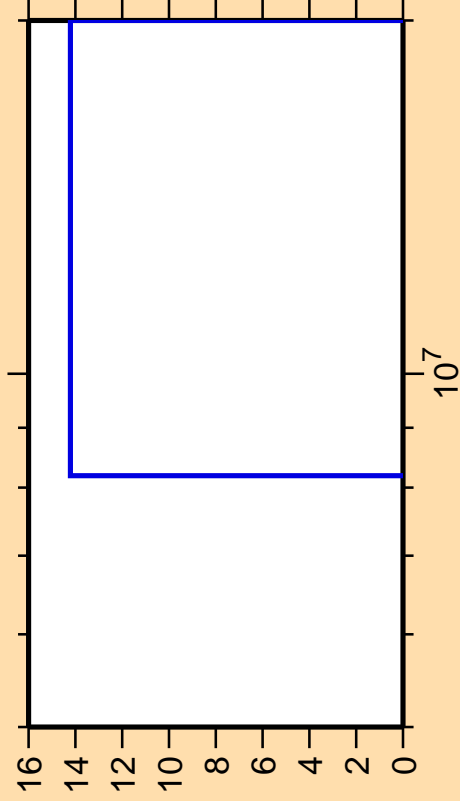
\Delta\sigma/\sigma vs. E for ^{237}\text{Bk}(n,f)
