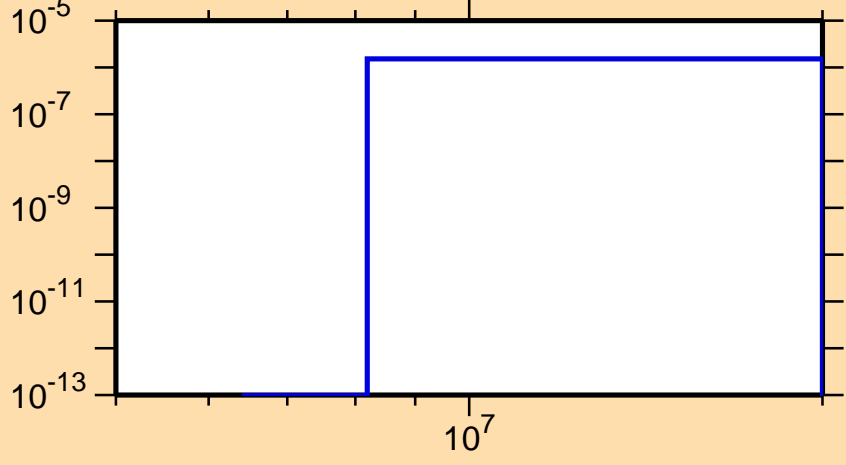
\sigma vs. E for ^{237}\text{Bk}(n,t)
