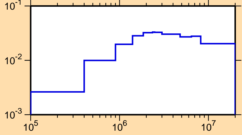
\sigma vs. E for ^{237}\text{Bk}(n,\text{inel.})
