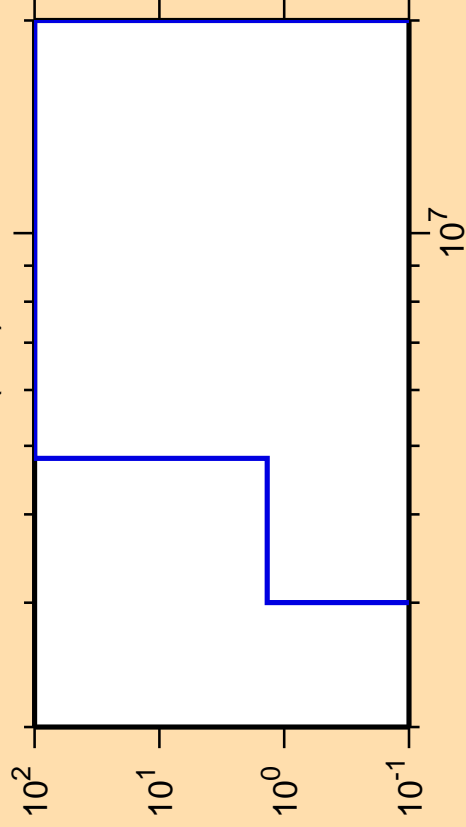
\Delta\sigma/\sigma vs. E for ^{237}\text{Bk}(n,d)
