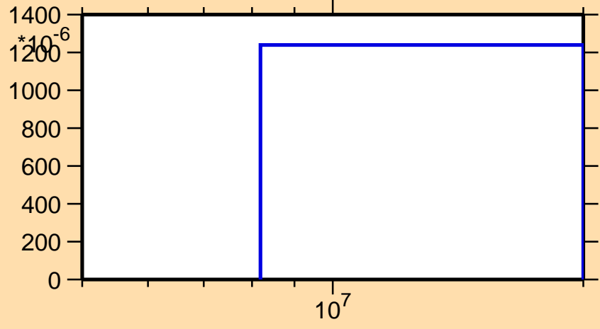
\sigma vs. E for ^{237}\text{Bk}(n,2n)
