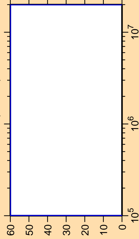
\Delta\sigma/\sigma vs. E for ^{237}\text{Bk}(n,\text{inel.})
