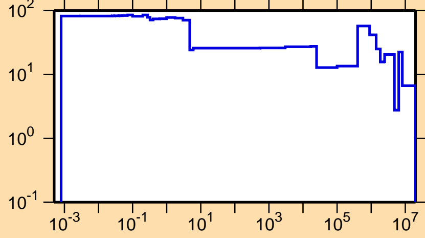
\Delta\sigma/\sigma vs. E for ^{237}\text{Bk}(n,\text{el.})
