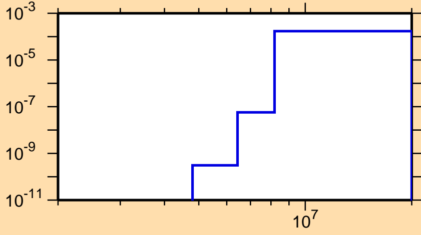
\sigma vs. E for ^{237}\text{Bk}(n,d)
