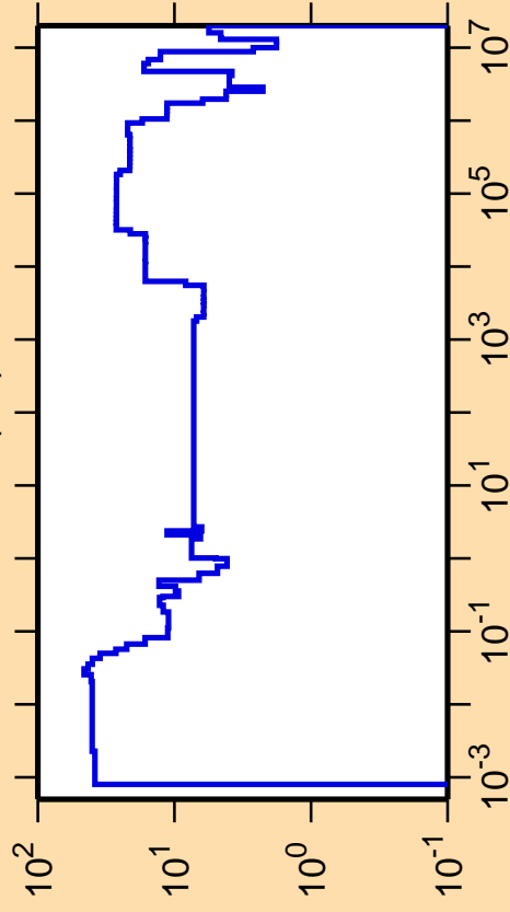
\Delta\sigma/\sigma vs. E for ^{238}\text{Bk}(n,f)
