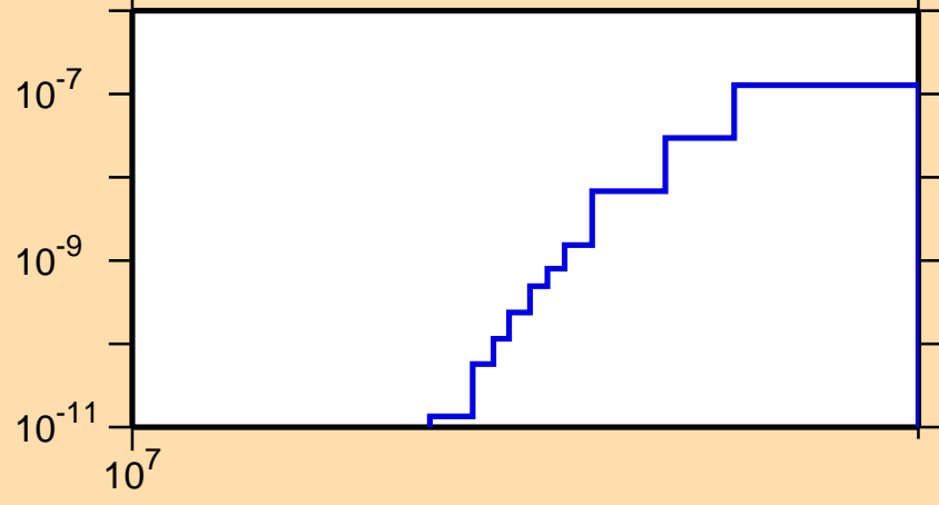
\sigma vs. E for ^{238}\text{Bk}(n,2np)
