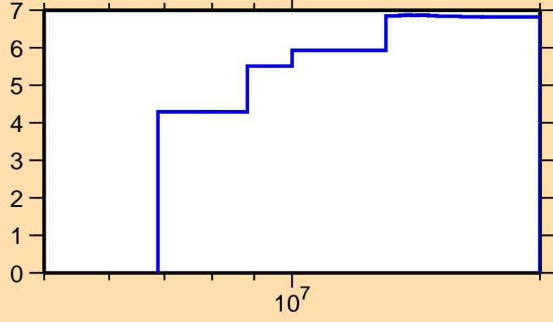
\Delta\sigma/\sigma vs. E for ^{238}\text{Bk}(n,\text{nonel.})
