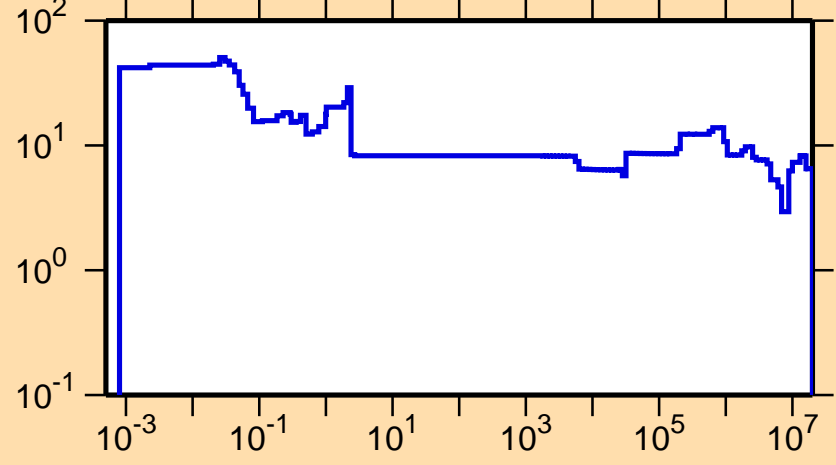
\Delta\sigma/\sigma vs. E for ^{238}\text{Bk}(n,tot.)
