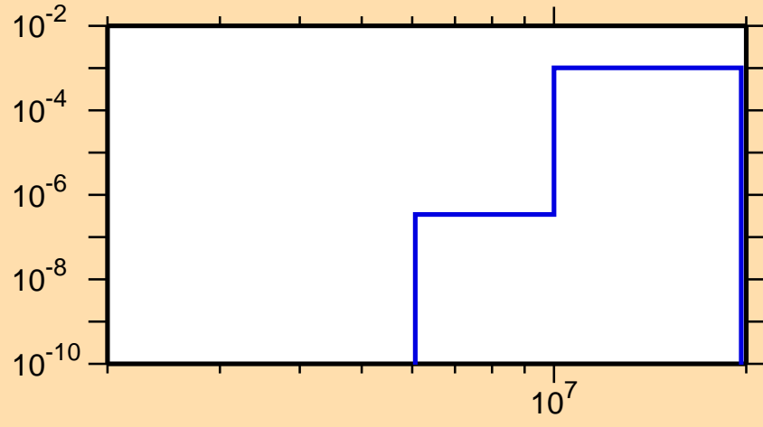
\sigma vs. E for ^{238}\text{Bk}(n,d)
