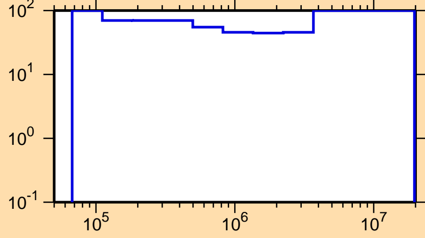
\Delta\sigma/\sigma vs. E for ^{238}\text{Bk}(n,\text{inel.})
