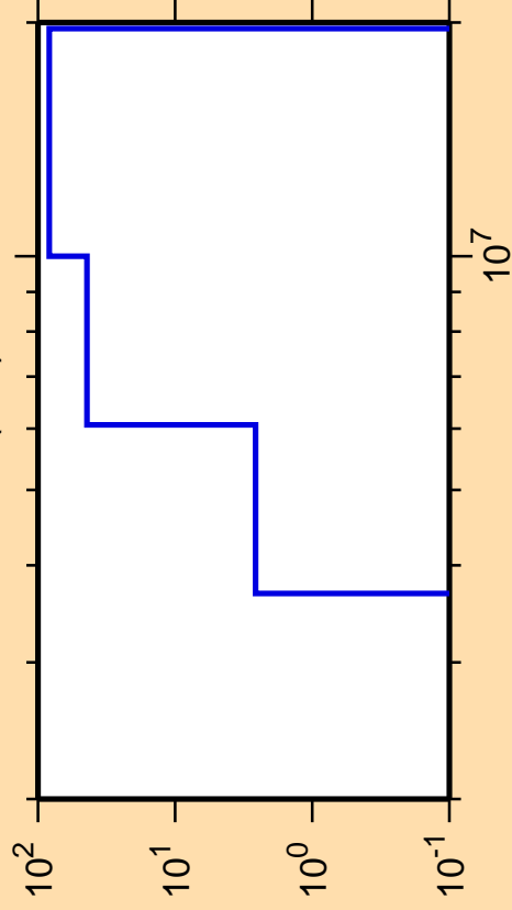
\Delta\sigma/\sigma vs. E for ^{238}\text{Bk}(n,d)
