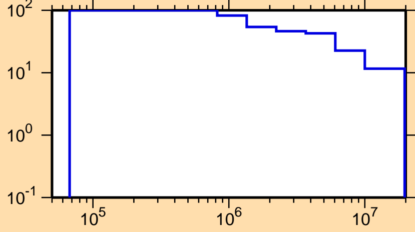
\Delta\sigma/\sigma vs. E for ^{238}\text{Bk}(n,n_1)
