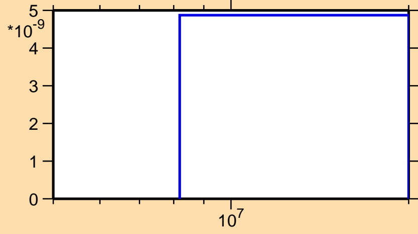
\sigma vs. E for ^{238}\text{Bk}(n,nd)
