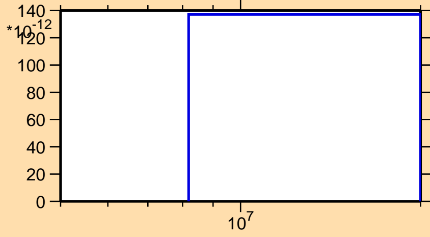
\sigma vs. E for ^{238}\text{Bk}(n,2n\alpha)
