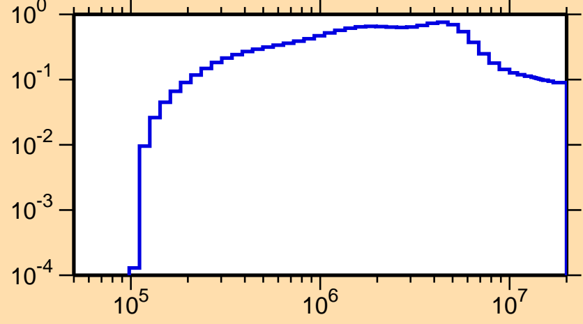
\sigma vs. E for ^{239}\text{Bk}(n,\text{inel.})
