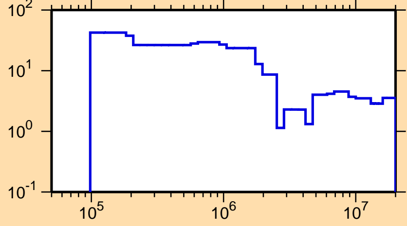
\Delta\sigma/\sigma vs. E for ^{239}\text{Bk}(n,\text{nonel.})
