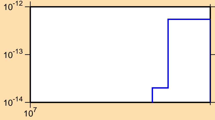
\sigma vs. E for ^{239}\text{Bk}(n,3n\alpha)
