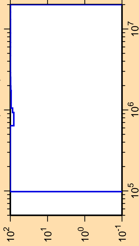
\Delta\sigma/\sigma vs. E for ^{239}\text{Bk}(n,\text{inel.})
