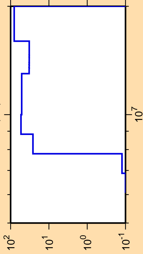
\Delta\sigma/\sigma vs. E for ^{239}\text{Bk}(n,t)
