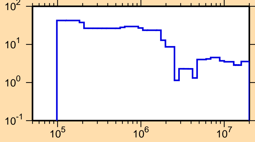
\Delta\sigma/\sigma vs. E for ^{239}\text{Bk}(n,n_{\text{nonel}}) .
