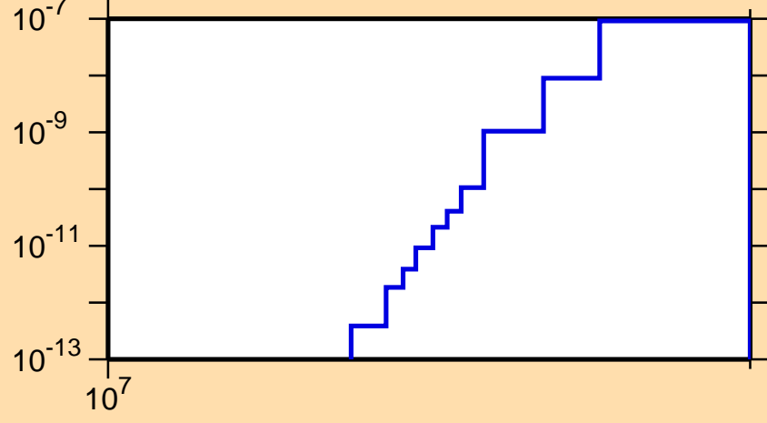
\sigma vs. E for ^{239}\text{Bk}(n,nd)
