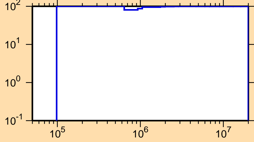
\Delta\sigma/\sigma vs. E for ^{239}\text{Bk}(n,\text{inel.})
