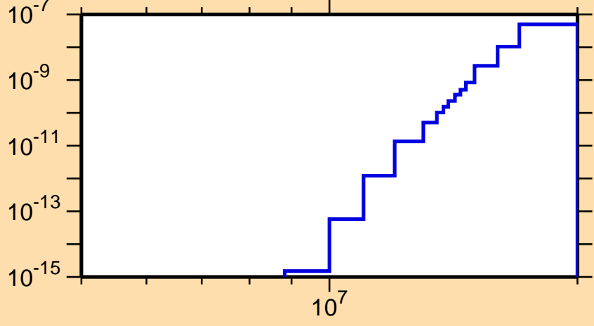
\sigma vs. E for ^{239}\text{Bk}(n,\text{He3})
