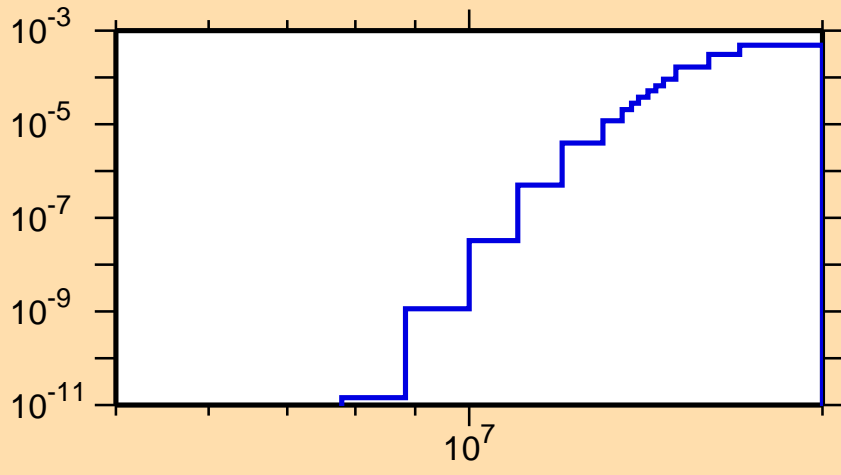
\sigma vs. E for ^{239}\text{Bk}(n,t)
