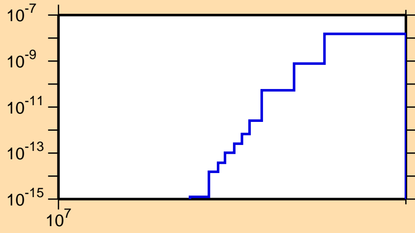
\sigma vs. E for ^{239}\text{Bk}(n,nt)
