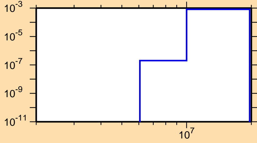
\sigma vs. E for ^{239}\text{Bk}(n,d)
