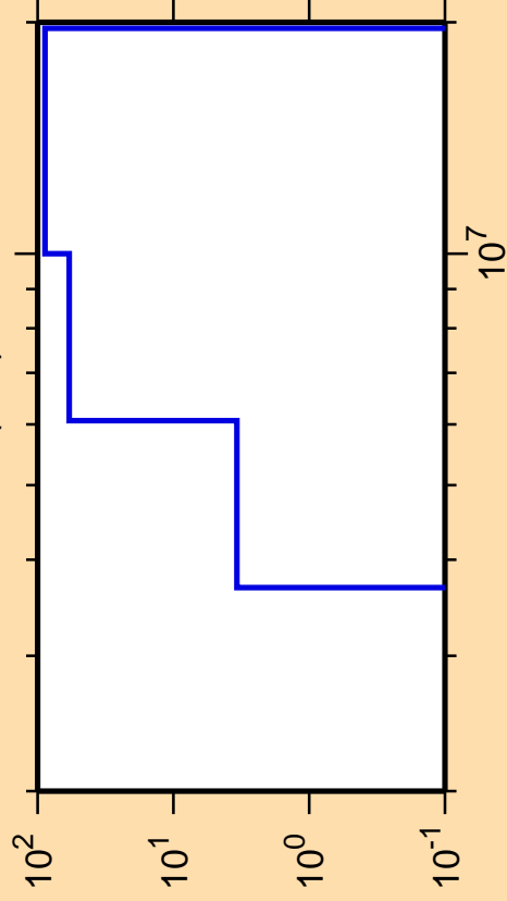
\Delta\sigma/\sigma vs. E for ^{239}\text{Bk}(n,d)
