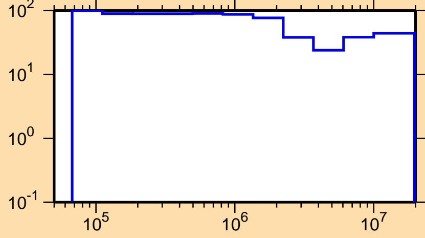
\Delta\sigma/\sigma vs. E for ^{239}\text{Bk}(n,n_1)
