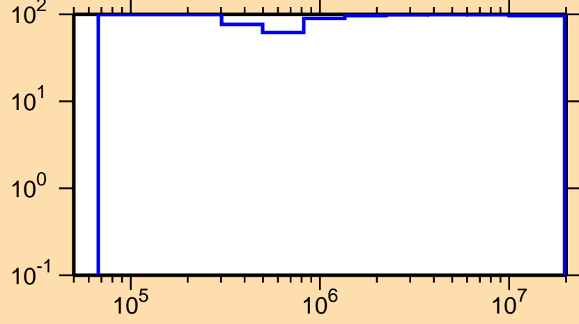
\Delta\sigma/\sigma vs. E for ^{239}\text{Bk}(n,n\text{cont.})
