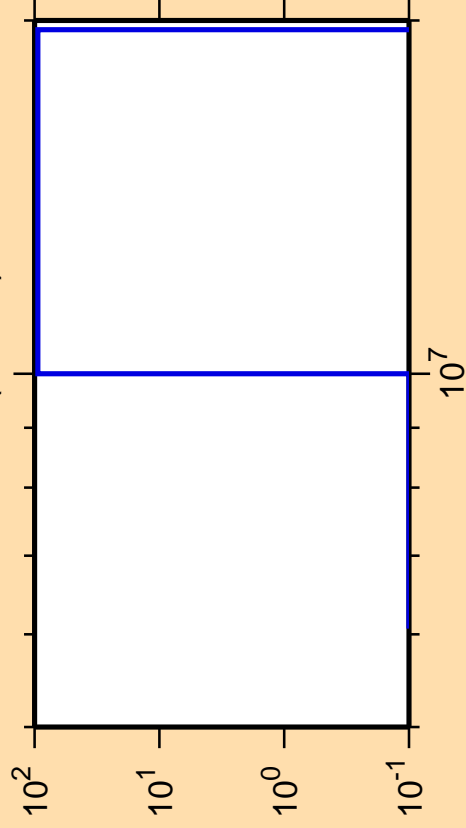
\Delta\sigma/\sigma vs. E for ^{239}\text{Bk}(n,2n\alpha)
