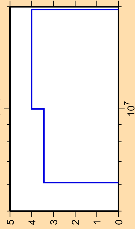
\Delta\sigma/\sigma vs. E for ^{239}\text{Bk}(n,f)
