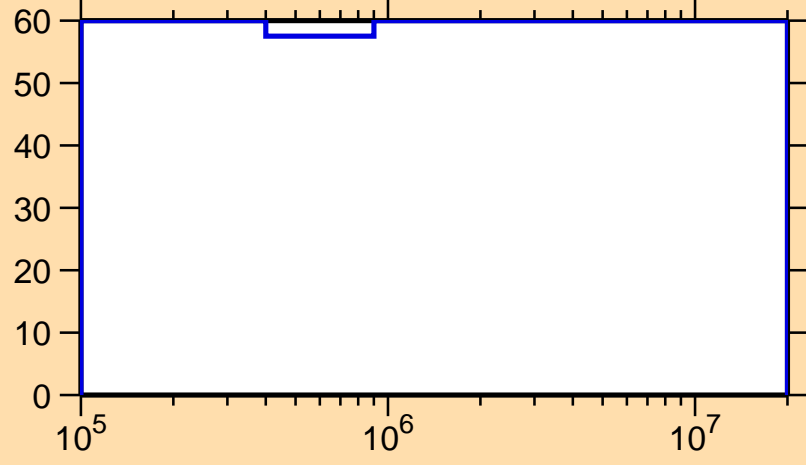
\Delta\sigma/\sigma vs. E for ^{239}\text{Bk}(n,ncont.)
