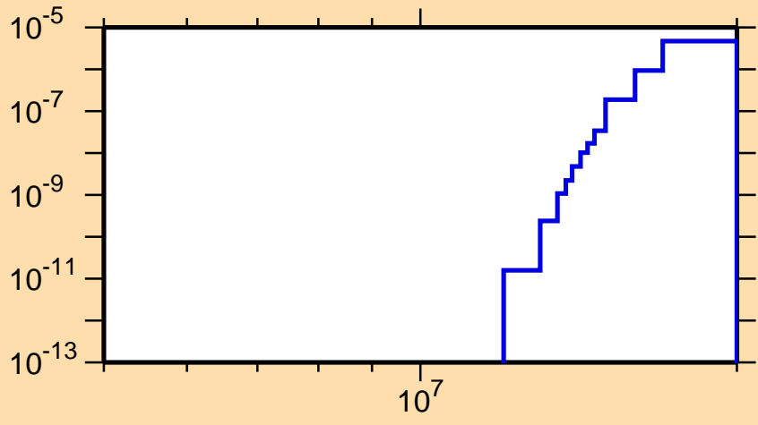
\sigma vs. E for ^{240}\text{Bk}(n,2np)
