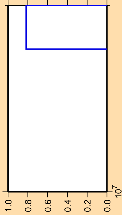
\Delta\sigma/\sigma vs. E for ^{240}\text{Bk} (mt 34)
