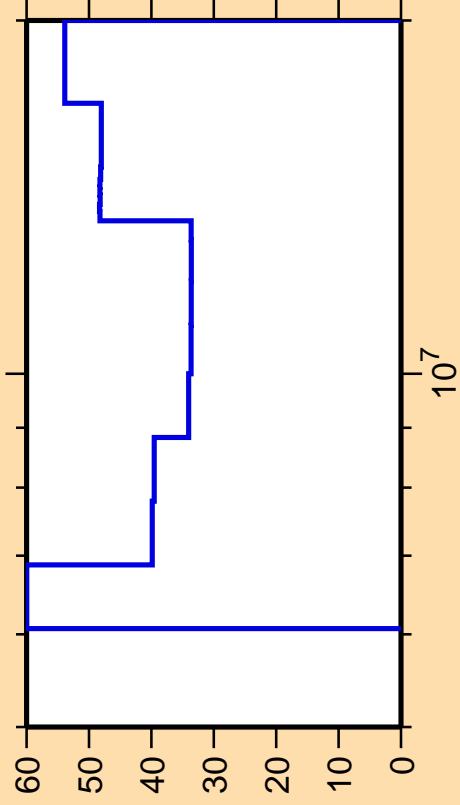
\Delta\sigma/\sigma vs. E for ^{240}\text{Bk}(n,p)
