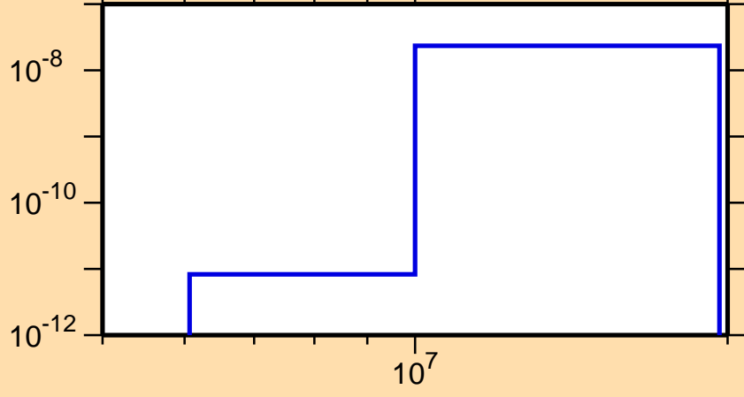
\sigma vs. E for ^{240}\text{Bk}(n,2n\alpha)
