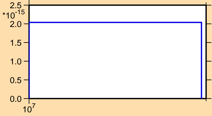
\sigma vs. E for ^{240}\text{Bk} (mt 34)
