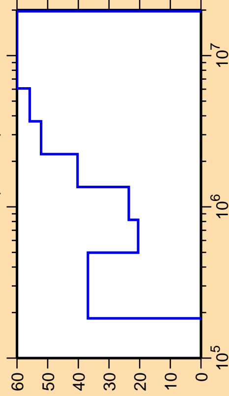
\Delta\sigma/\sigma vs. E for ^{240}\text{Bk}(n,\text{inel.})
