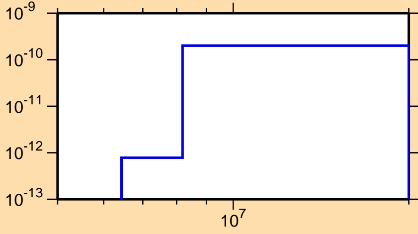
\sigma vs. E for ^{240}\text{Bk}(n,p\alpha)
