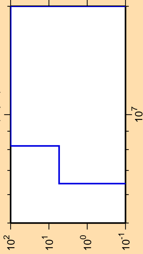
\Delta\sigma/\sigma vs. E for ^{240}\text{Bk}(n,p\alpha)
