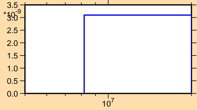
\sigma vs. E for ^{240}\text{Bk}(n,\text{He3})
