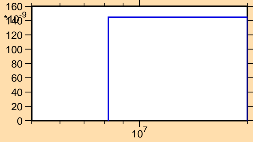
\sigma vs. E for ^{240}\text{Bk}(n,\text{nd})
