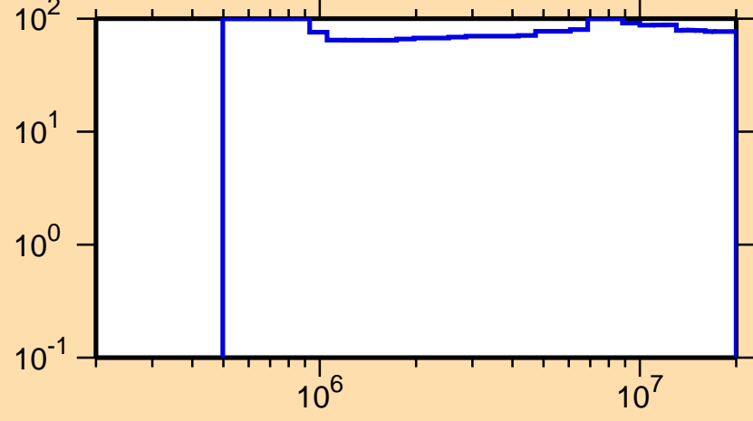
\Delta\sigma/\sigma vs. E for ^{241}\text{Bk}(n,n\text{cont.})
