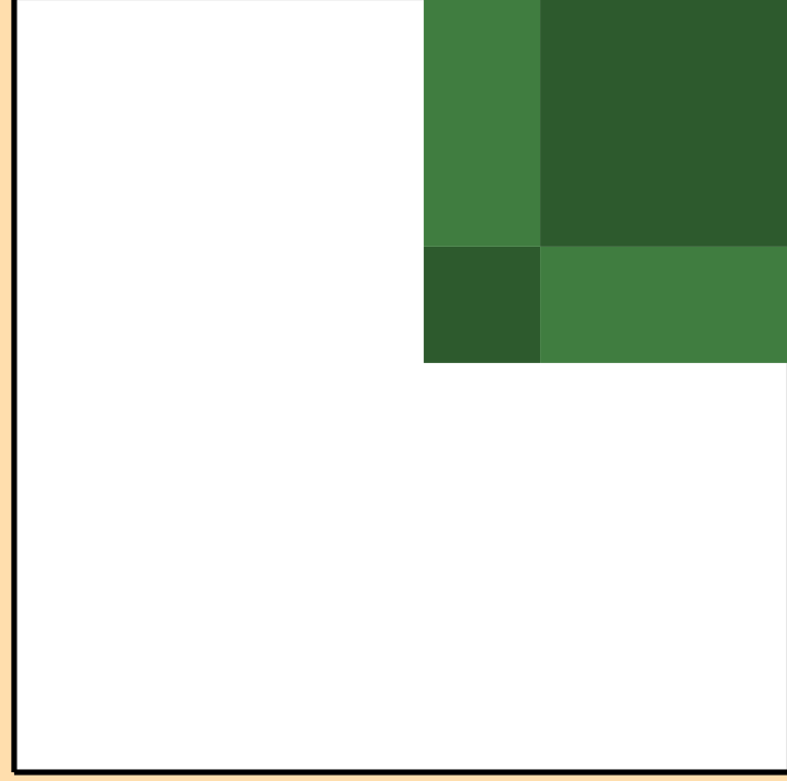
\sigma vs. E for ^{241}\text{Bk}(n,3n)
