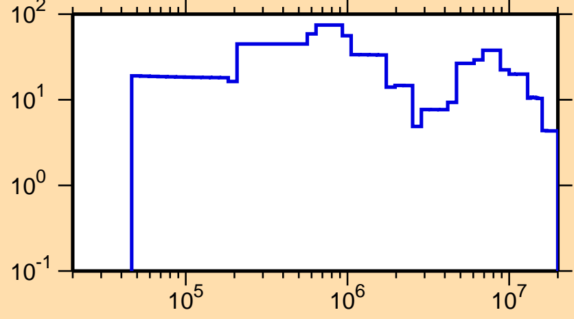
\Delta\sigma/\sigma vs. E for ^{241}\text{Bk}(n,\text{el.})
