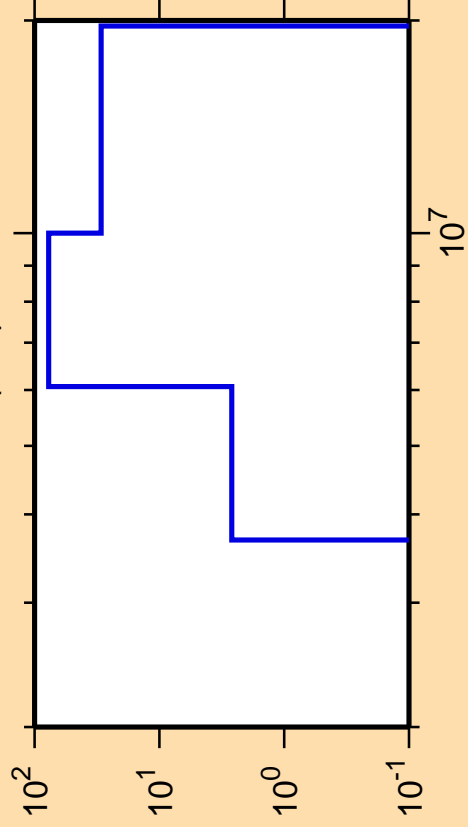
\Delta\sigma/\sigma vs. E for ^{241}\text{Bk}(n,d)
