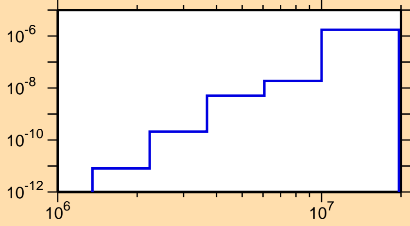
\sigma vs. E for ^{241}\text{Bk}(n,n\alpha)
