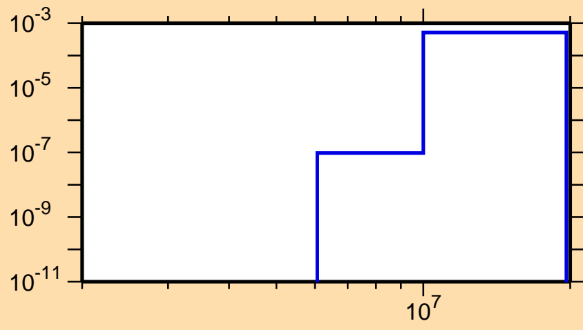
\sigma vs. E for ^{241}\text{Bk}(n,d)
