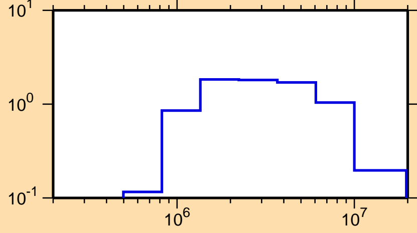
\sigma vs. E for ^{241}\text{Bk}(n,n\text{cont.})
