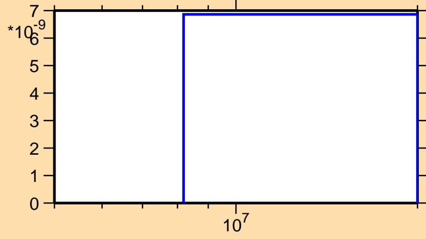
\sigma vs. E for ^{241}\text{Bk}(n,\text{nd})
