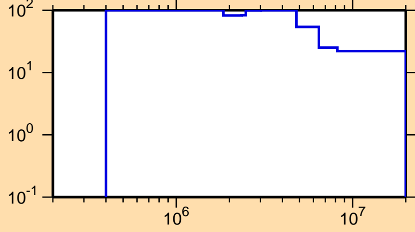
\Delta\sigma/\sigma vs. E for ^{241}\text{Bk}(n,f)
