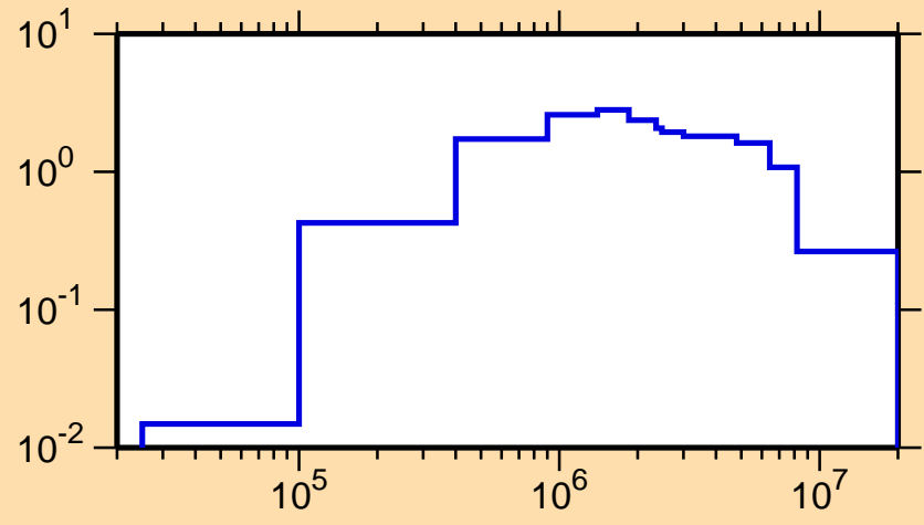
\sigma vs. E for ^{241}\text{Bk}(n,\text{inel.})
