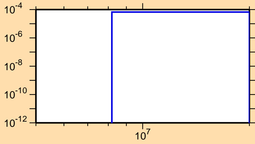
\sigma vs. E for ^{241}\text{Bk}(n,t)
