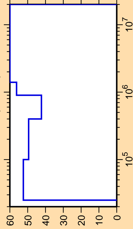
\Delta\sigma/\sigma vs. E for ^{241}\text{Bk}(n,\text{inel.})
